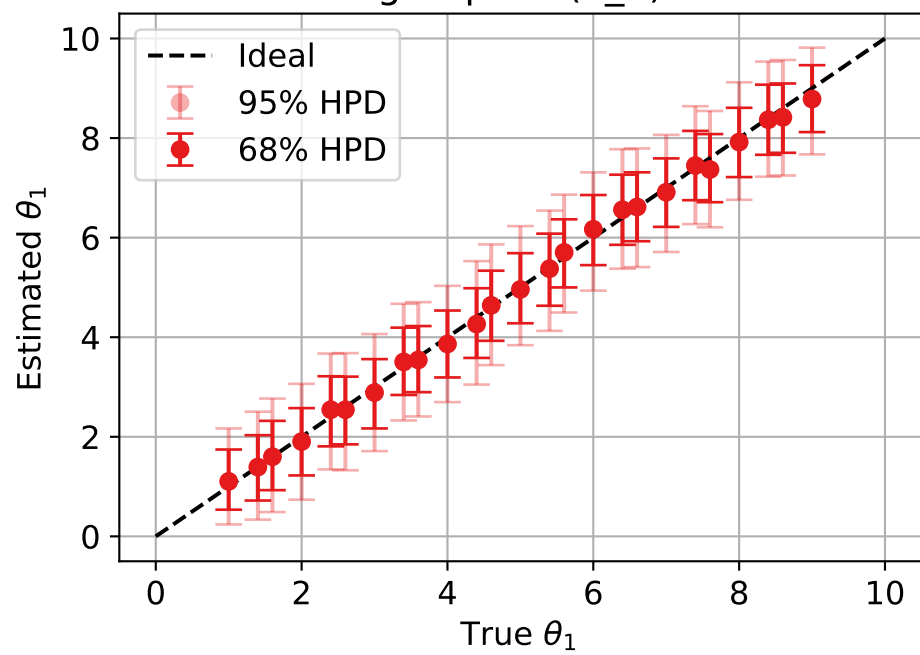
exponential prior ( \theta_1 )
