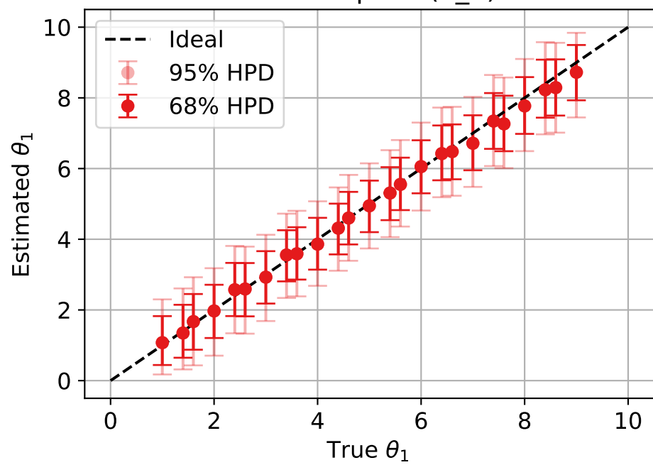
normal prior ( \theta_1 )
