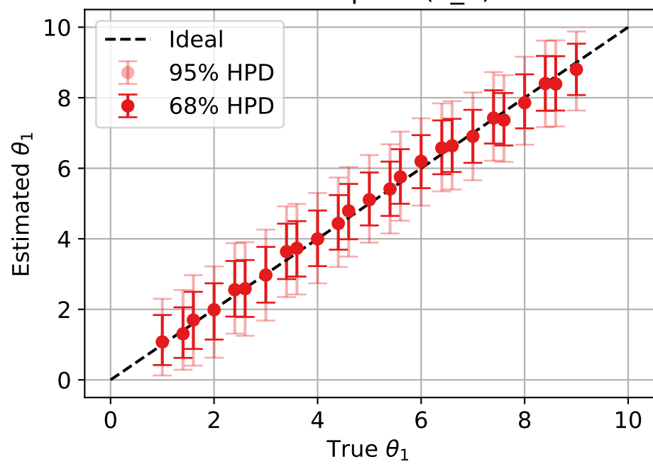
grid prior ( \theta_1 )
