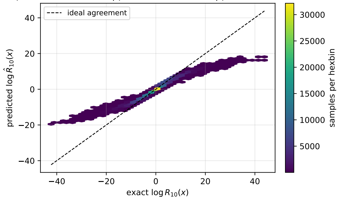
grid prior pooled RMSE=1.85 | pair median=0.784 | pair worst=10.1
