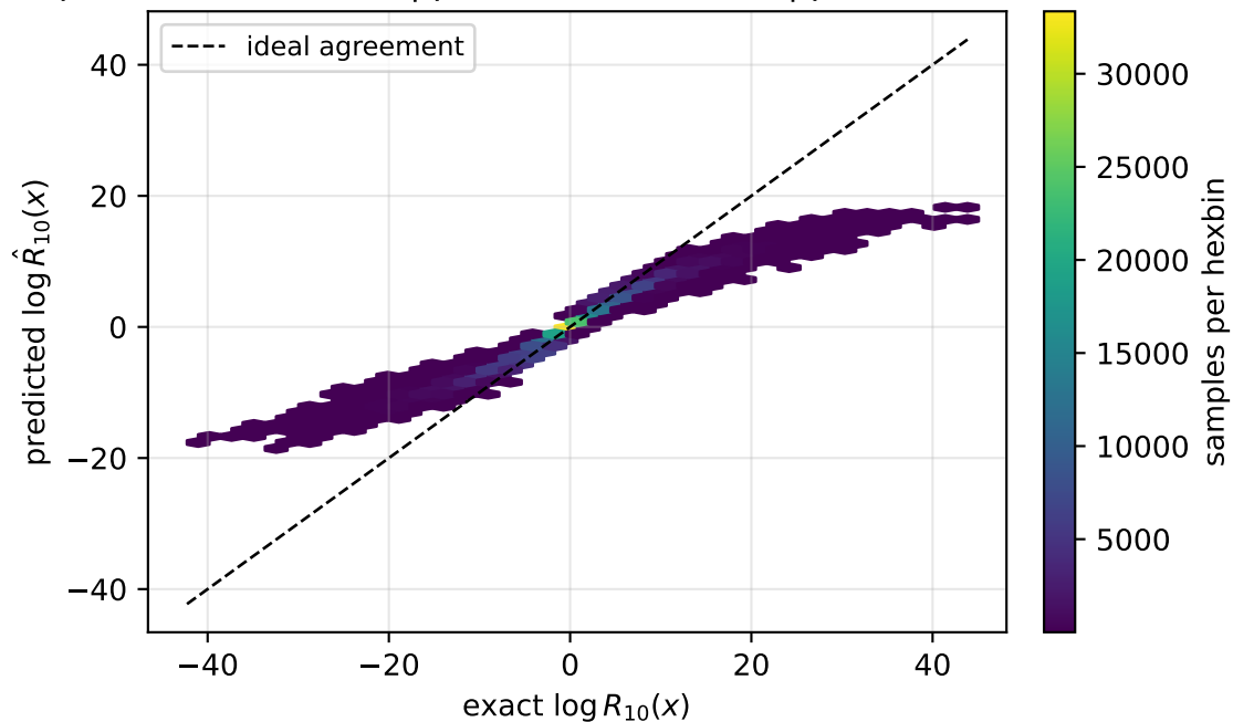
normal prior pooled RMSE=2.04 | pair median=0.851 | pair worst=10.6
