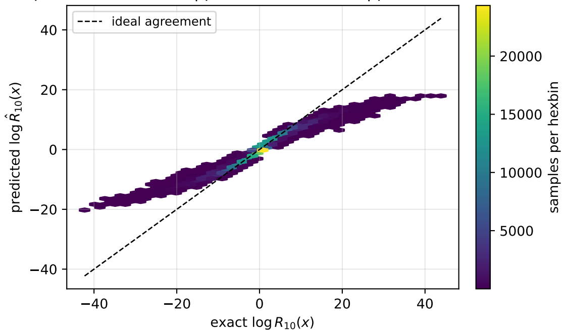
exponential prior pooled RMSE=1.82 | pair median=0.719 | pair worst=10
