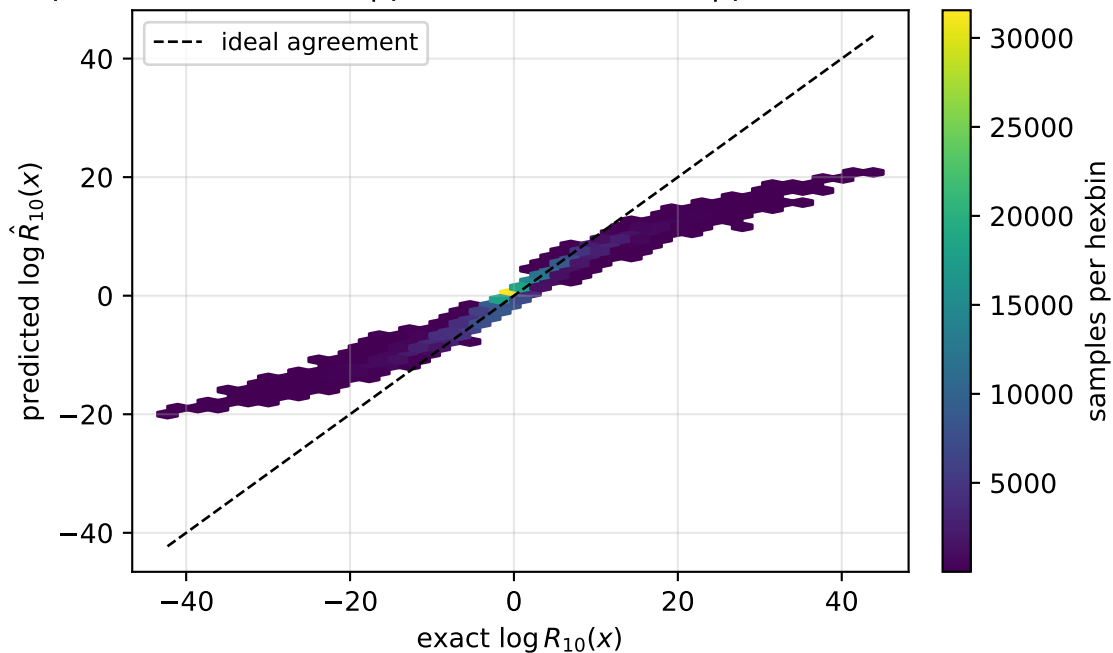
uniform prior pooled RMSE=1.78 | pair median=0.802 | pair worst=9.68
