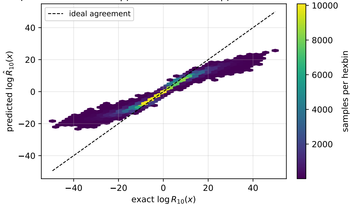
exponential prior pooled RMSE=4.21 | pair median=2.37 | pair worst=12.7
