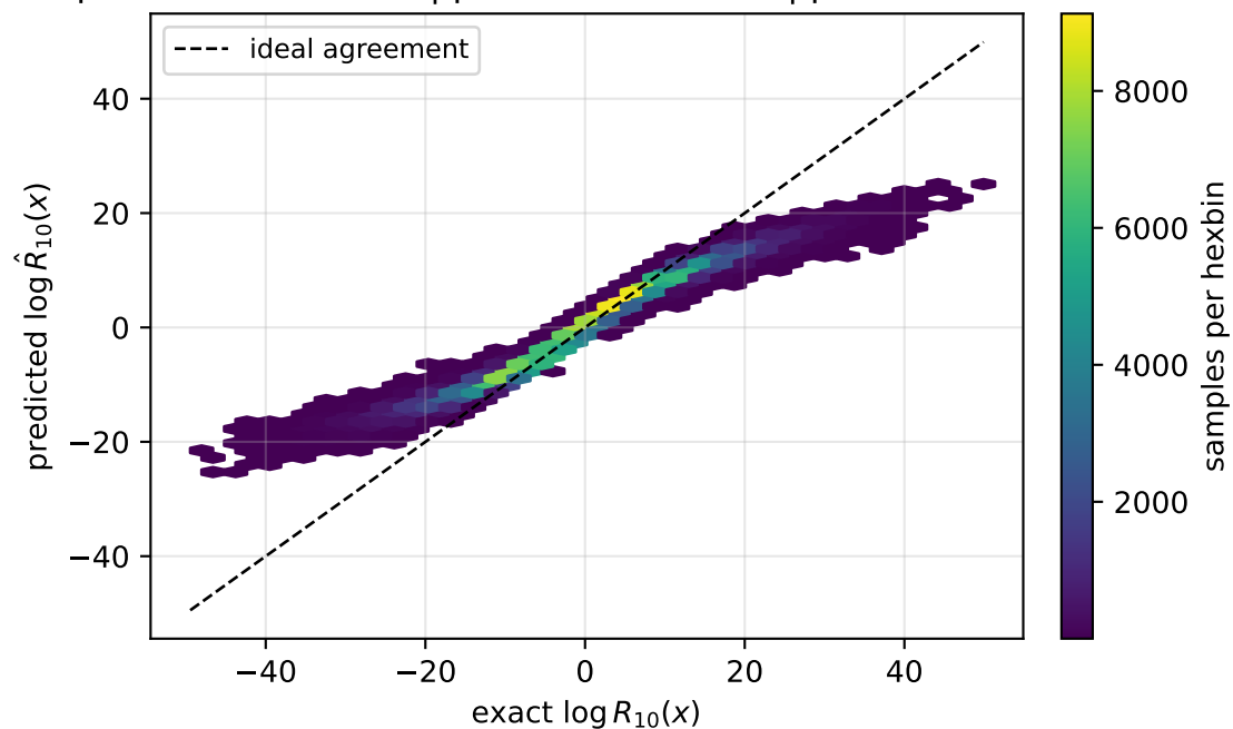
grid prior pooled RMSE=3.44 | pair median=1.77 | pair worst=10.9
