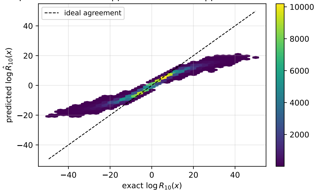
exponential prior pooled RMSE=4.21 | pair median=2.37 | pair worst=12.7
