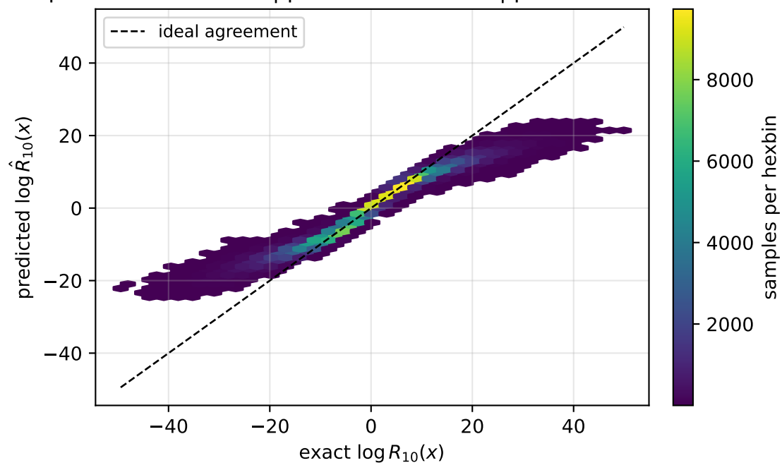
grid prior pooled RMSE=3.44 | pair median=1.77 | pair worst=10.9
