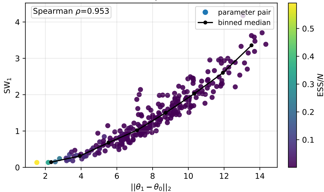
exponential prior median=1.27 | worst=4.1
