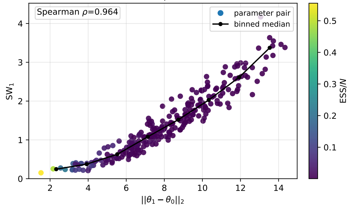
grid prior median=1.3 | worst=4.31
