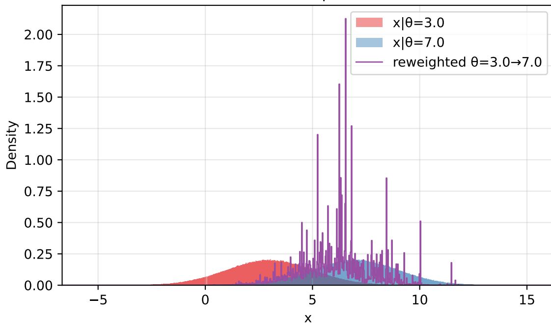
exponential prior N=1,000,000 | ESS=171
