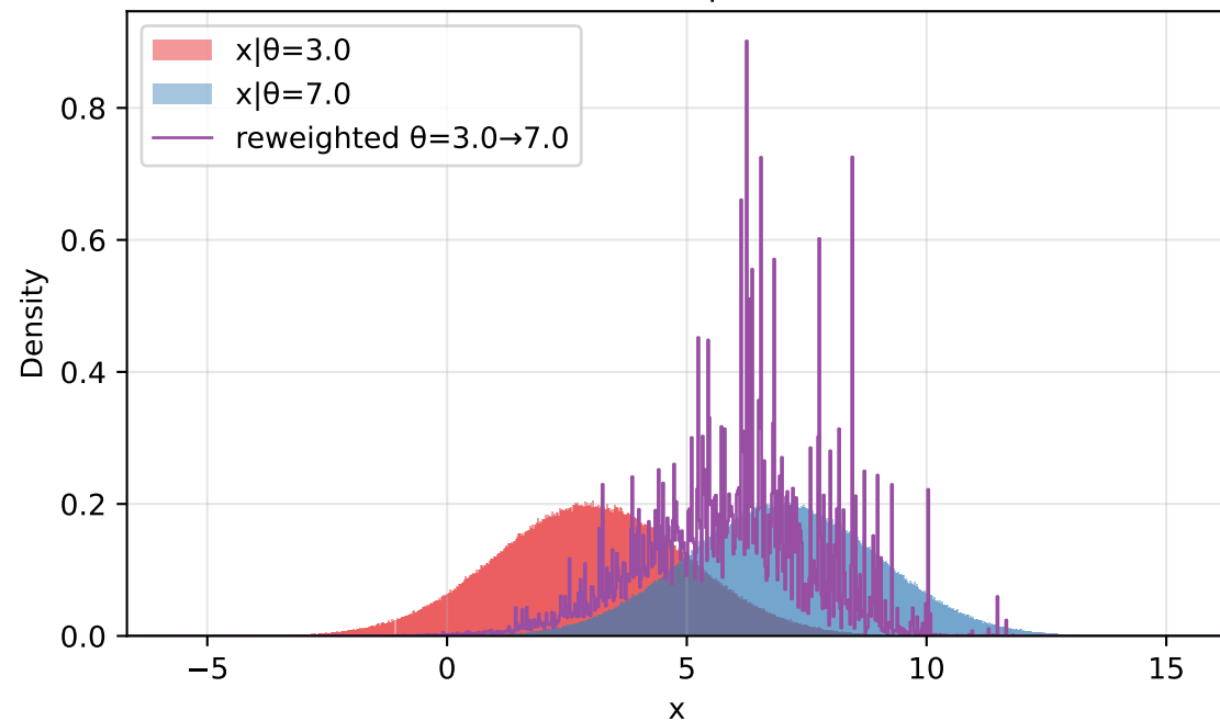
grid prior N=1,000,000 | ESS=134
