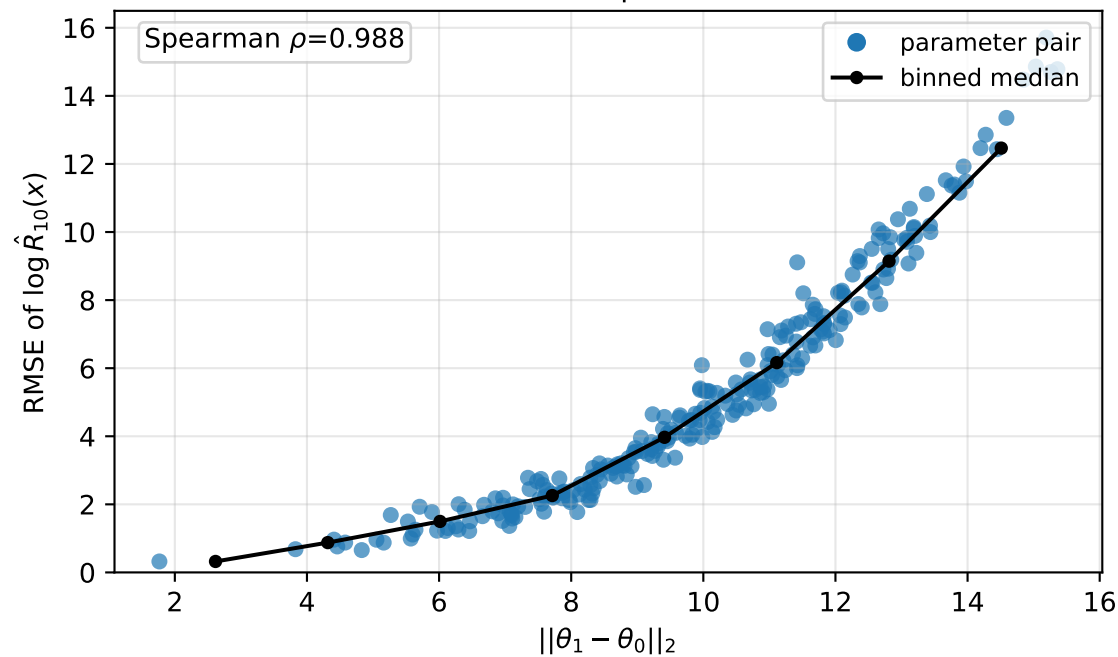
normal prior median=4.64 | worst=15.7
