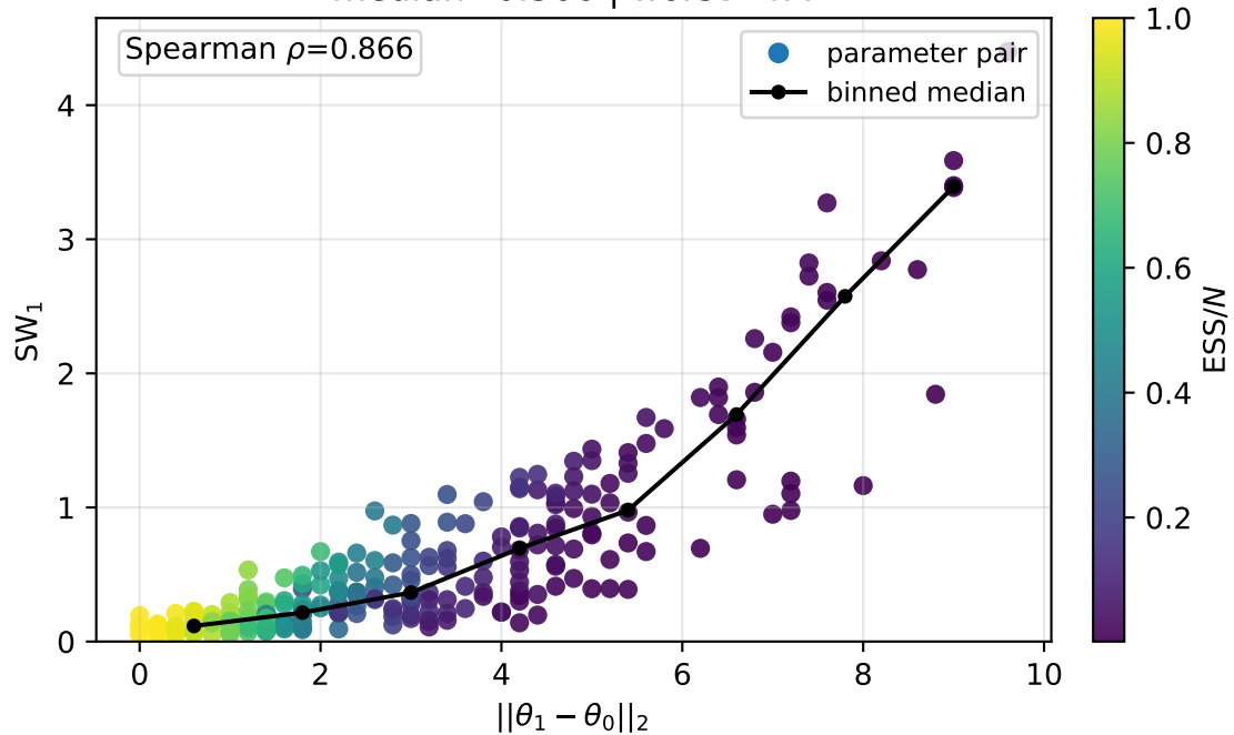
grid prior median=0.262 | worst=4.32
