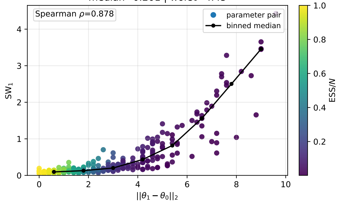
exponential prior median=0.201 | worst=4.43
