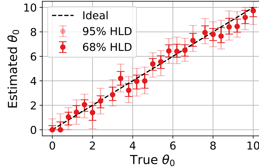
normal prior ( \theta_0 )
