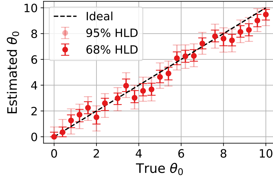
uniform prior ( \theta_0 )
