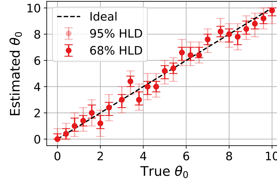
grid prior ( \theta_0 )
