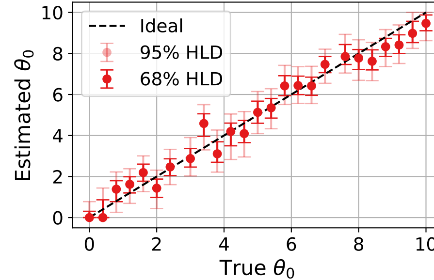
exponential prior ( \theta_0 )
