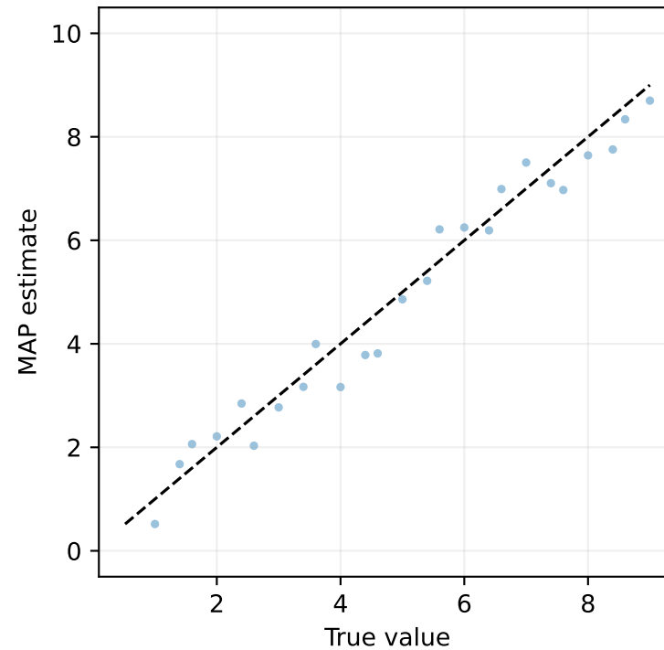
config_018 (1D)
