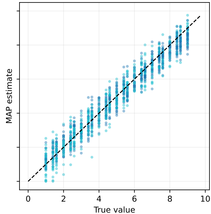
config_013 (2D)
