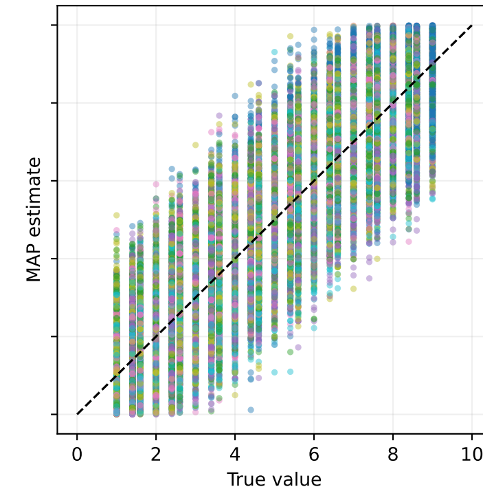
config_017 (6D)
