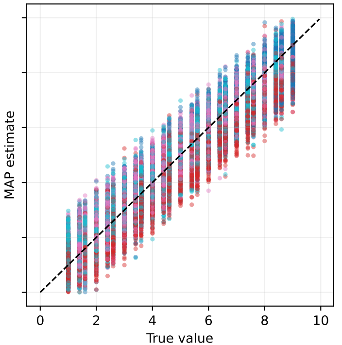
config_014 (4D)
