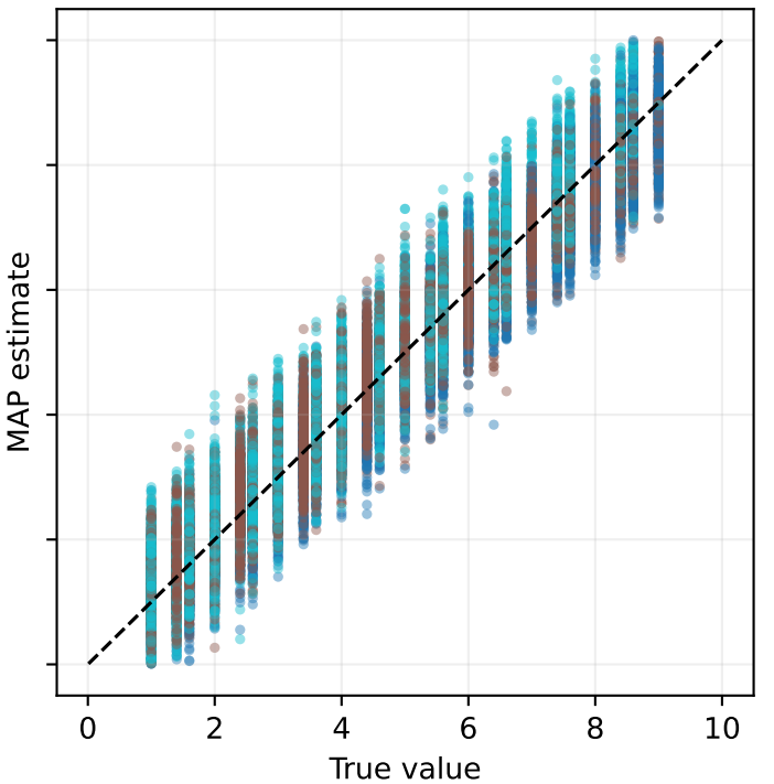
config_012 (3D)
