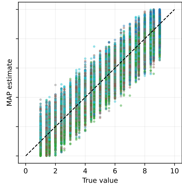
config_015 (5D)
