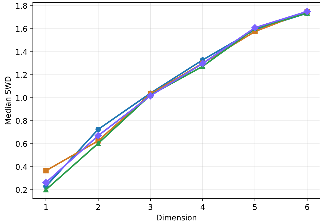
Median SWD
