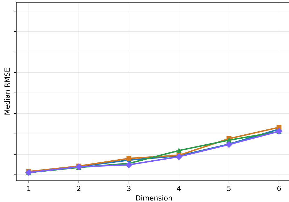
Median RMSE
