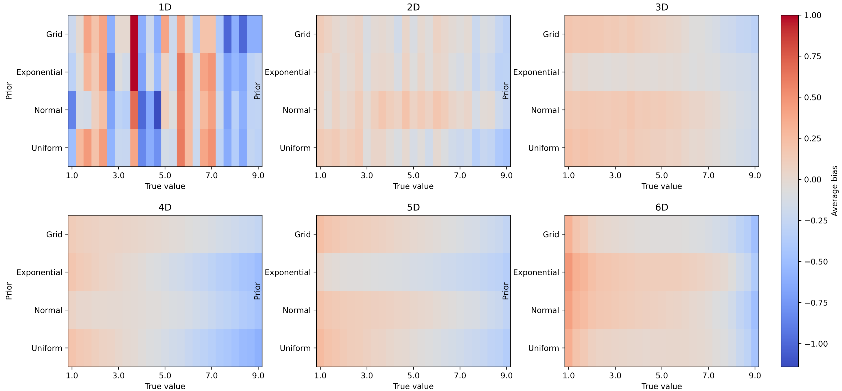
Bias heatmaps with prior rows
