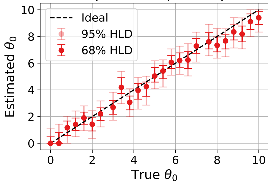
exponential prior ( \theta_0 )
