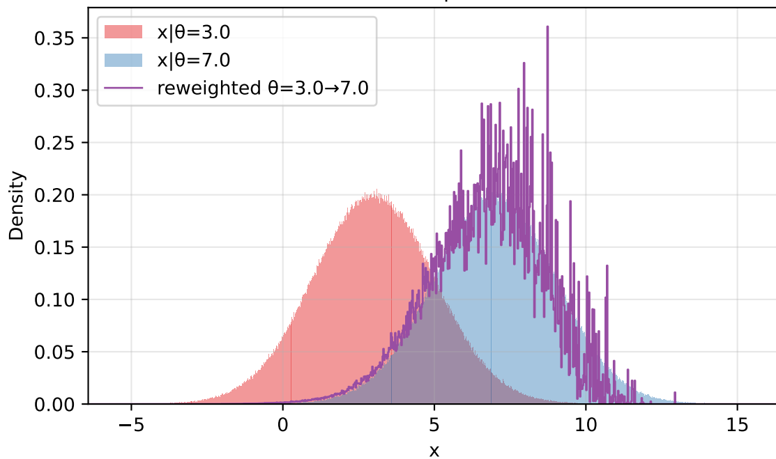
exponential prior N=1,000,000 | ESS=4,275
