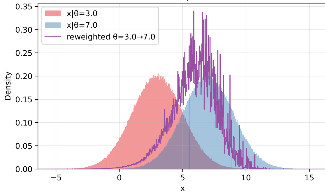
grid prior N=1,000,000 | ESS=5,081
