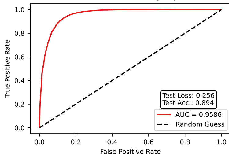
Test ROC Curve for 0. grid prior
