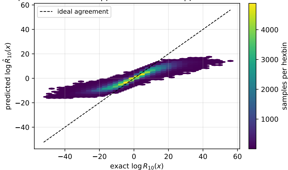
normal prior
