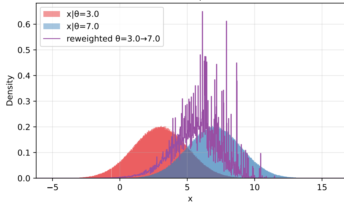
grid prior N=1,000,000 | ESS=151
