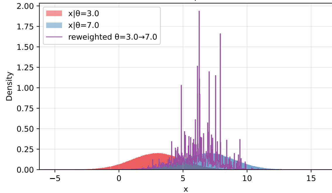
grid prior N=1,000,000 | ESS=151
