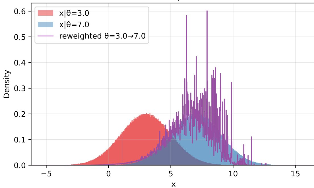
exponential prior N=1,000,000 | ESS=1,275
