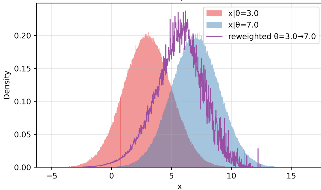
exponential prior N=1,000,000 | ESS=23,418
