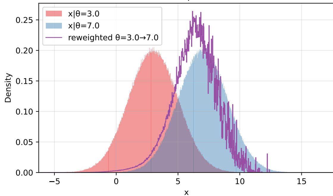
grid prior N=1,000,000 | ESS=17,433
