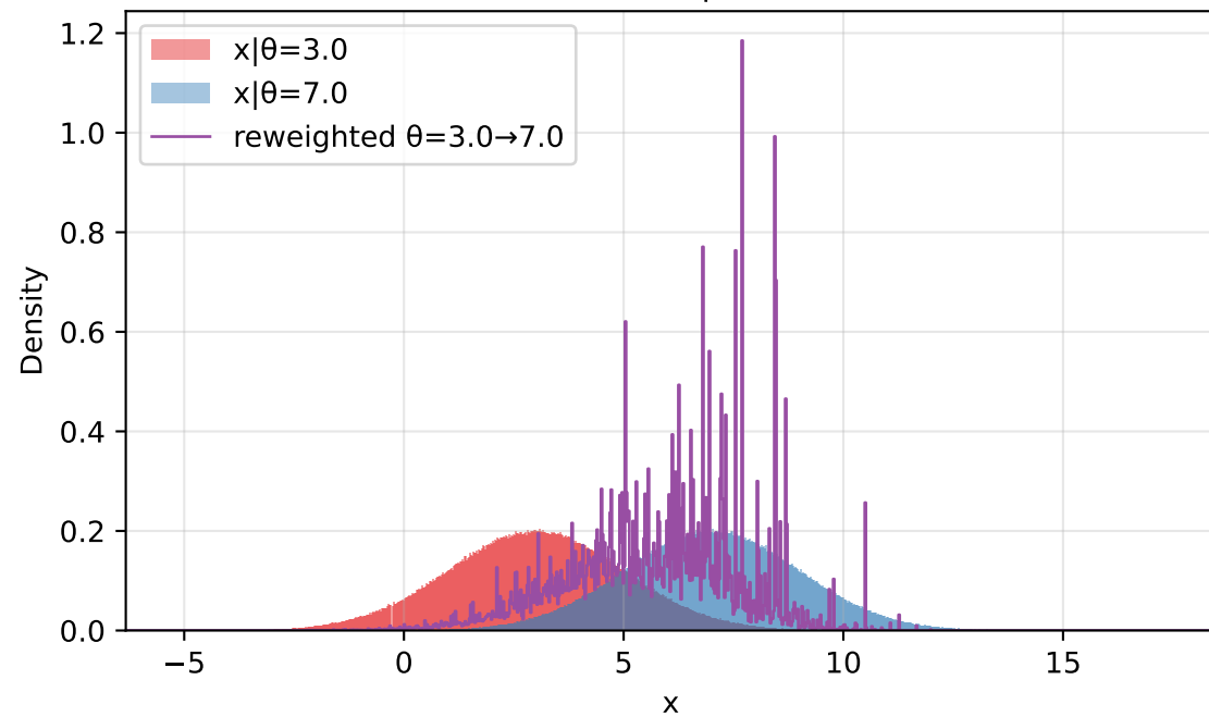
grid prior N=1,000,000 | ESS=341
