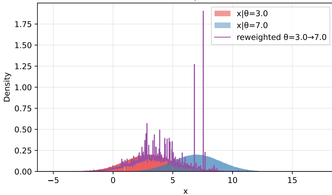
exponential prior N=1,000,000 | ESS=81
