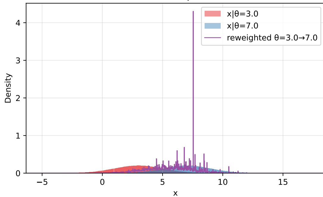
exponential prior N=1,000,000 | ESS=81
