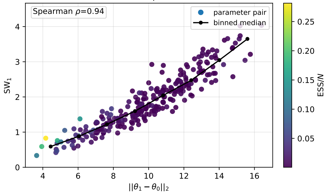
exponential prior median=1.81 | worst=4.04
