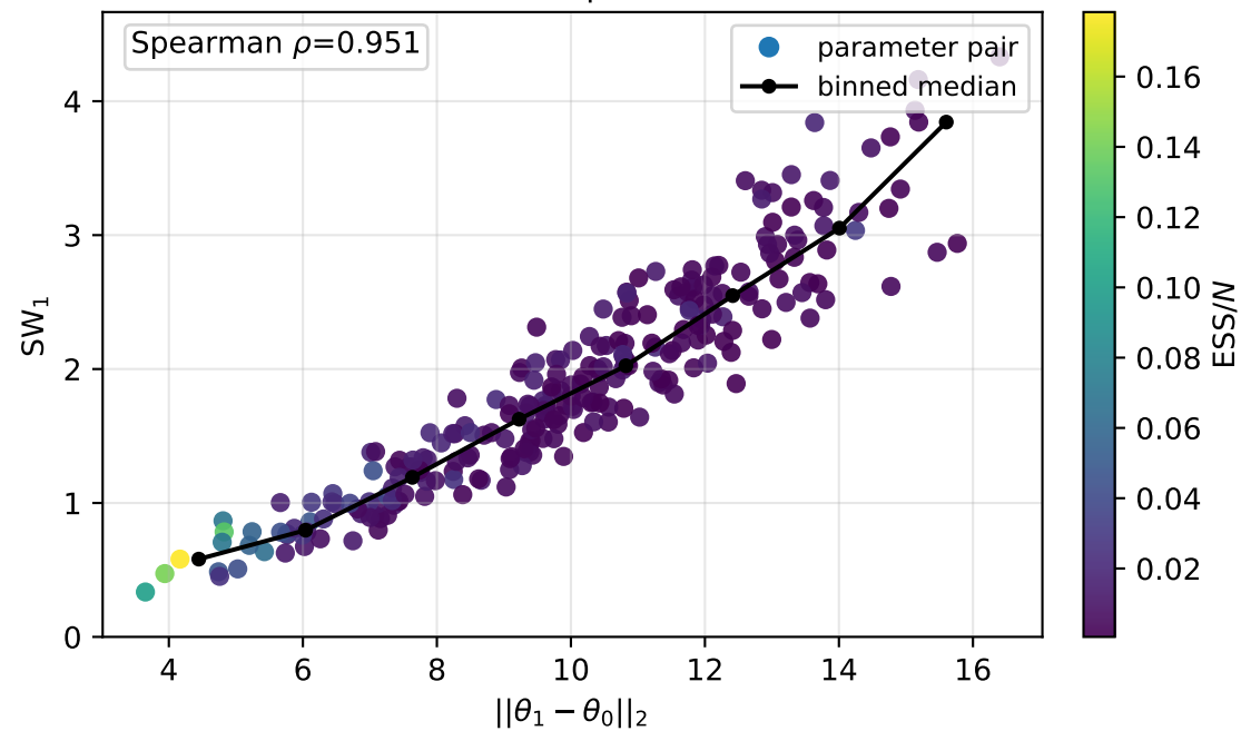
grid prior median=1.83 | worst=4.33
