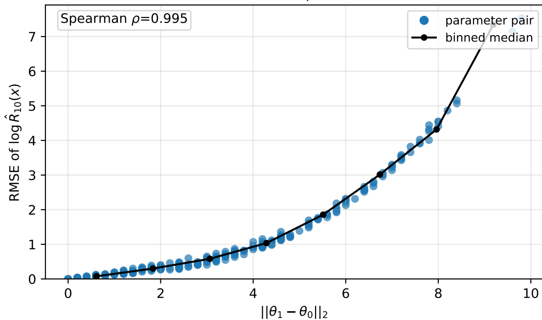
exponential prior median=0.473 | worst=6.72
