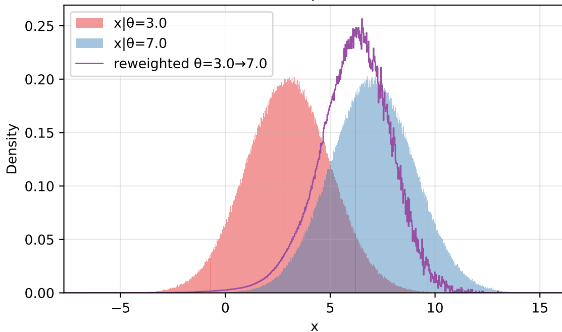
exponential prior N=1,000,000 | ESS=121,172
