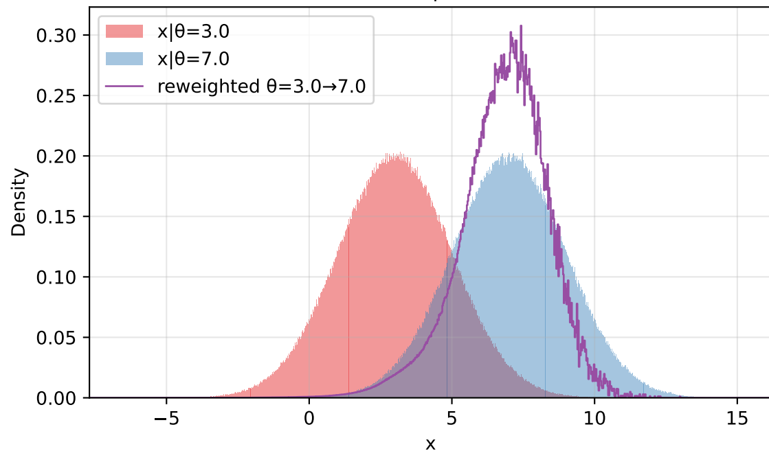
grid prior N=1,000,000 | ESS=86,536
