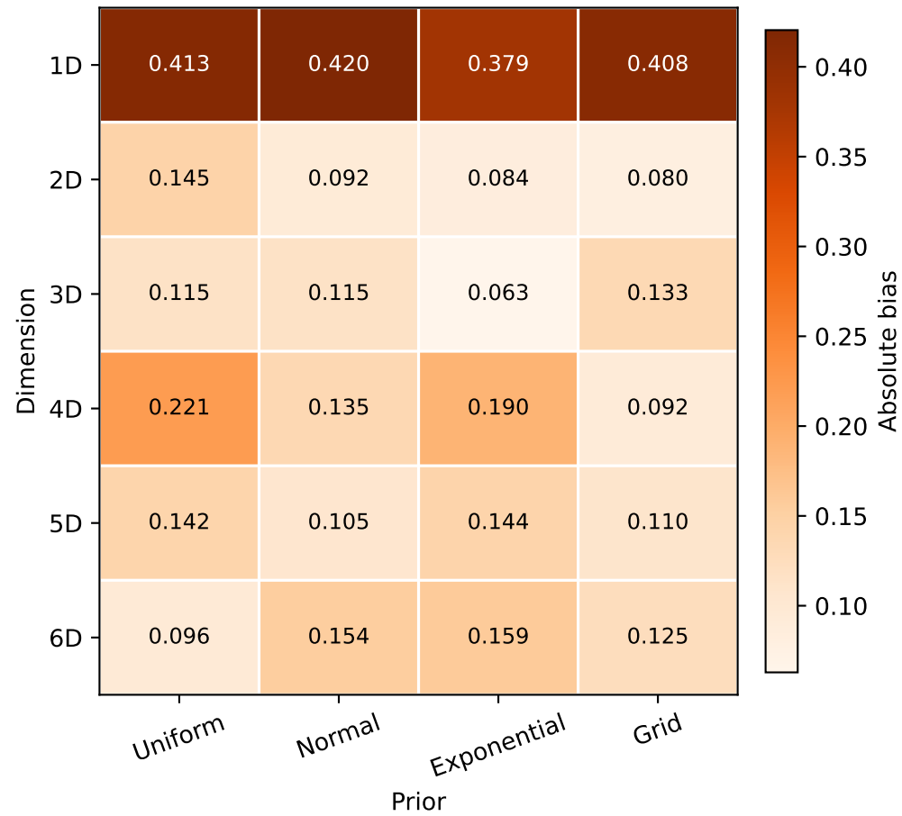
Mean absolute bias
