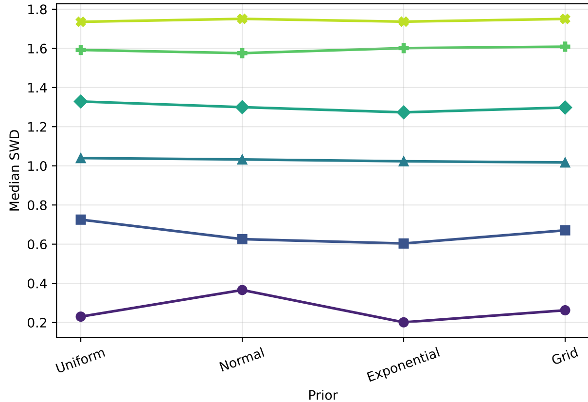
Median SWD by prior
