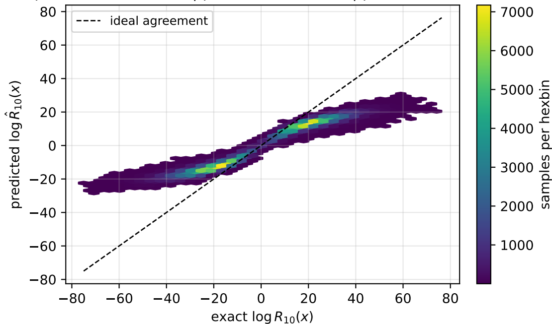
grid prior
