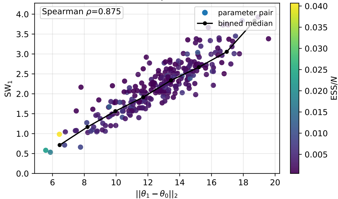
exponential prior median=2.22 | worst=3.93
