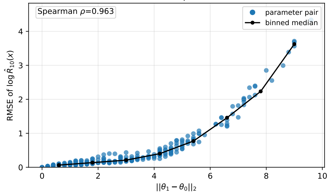
uniform prior median=0.213 | worst=4.34
