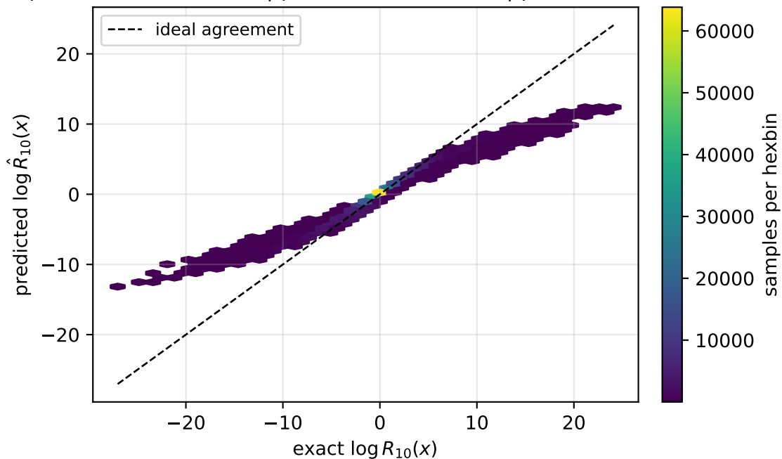
exponential prior pooled RMSE=0.885 | pair median=0.217 | pair worst=4.41
