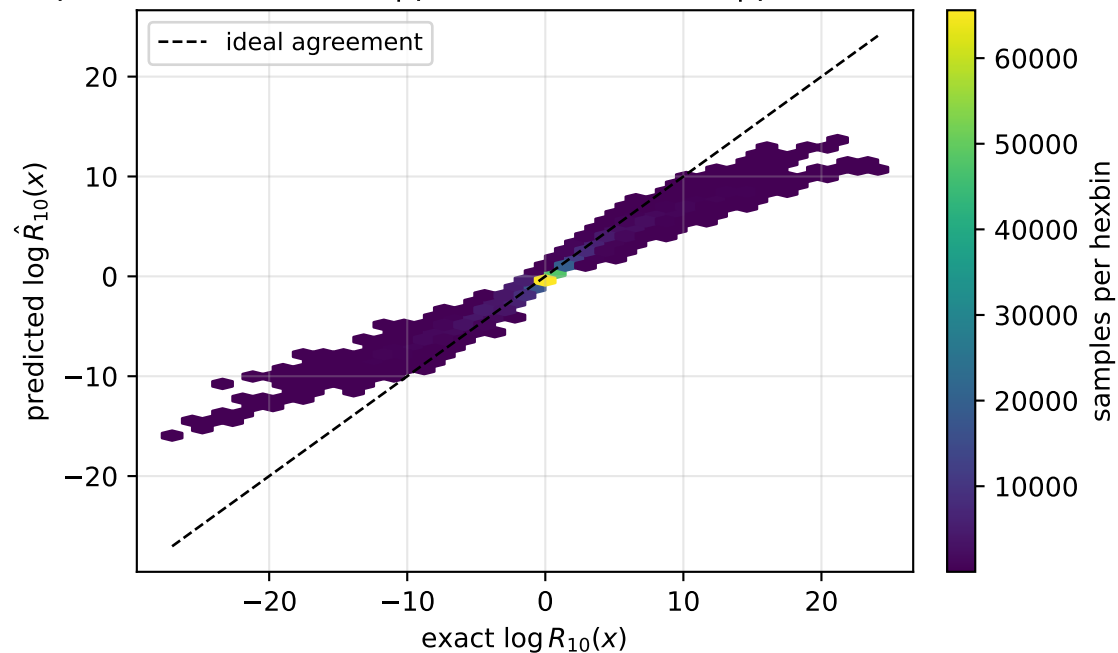
normal prior pooled RMSE=0.994 | pair median=0.319 | pair worst=4.6
