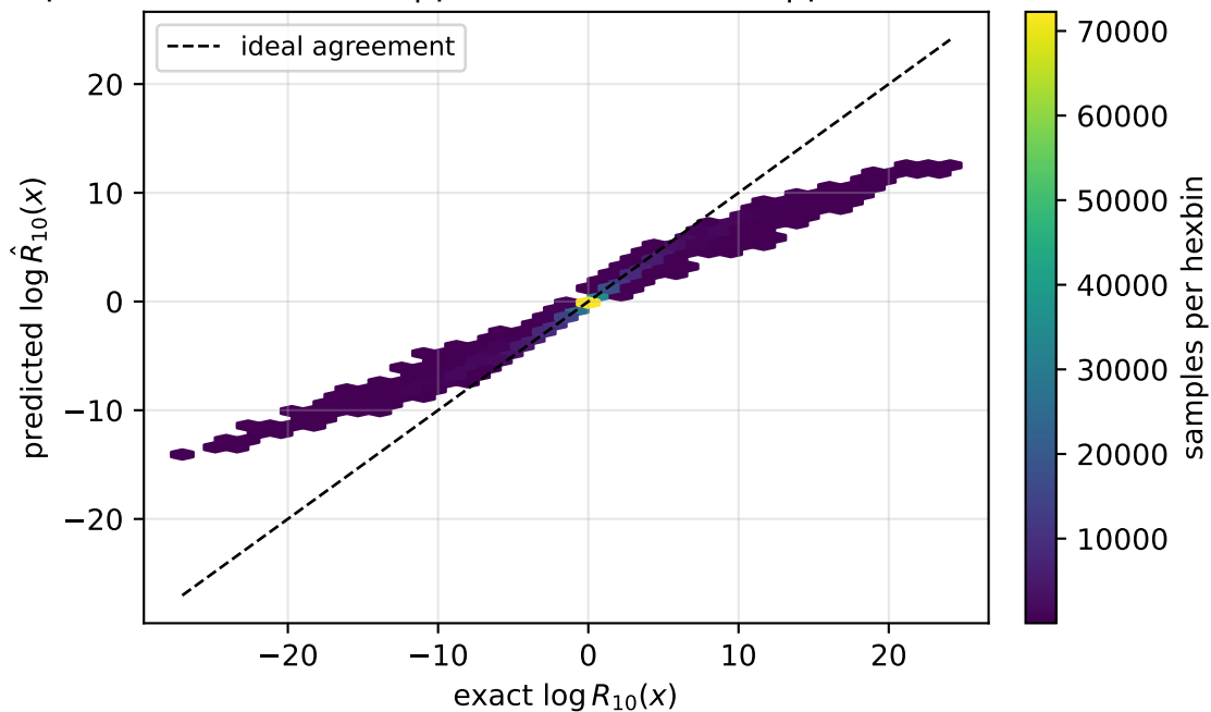
grid prior pooled RMSE=0.898 | pair median=0.223 | pair worst=4.42
