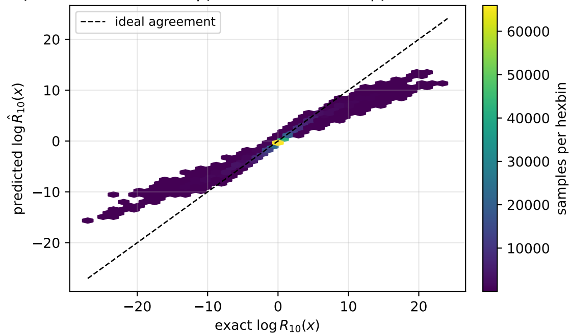
uniform prior pooled RMSE=0.871 | pair median=0.213 | pair worst=4.34
