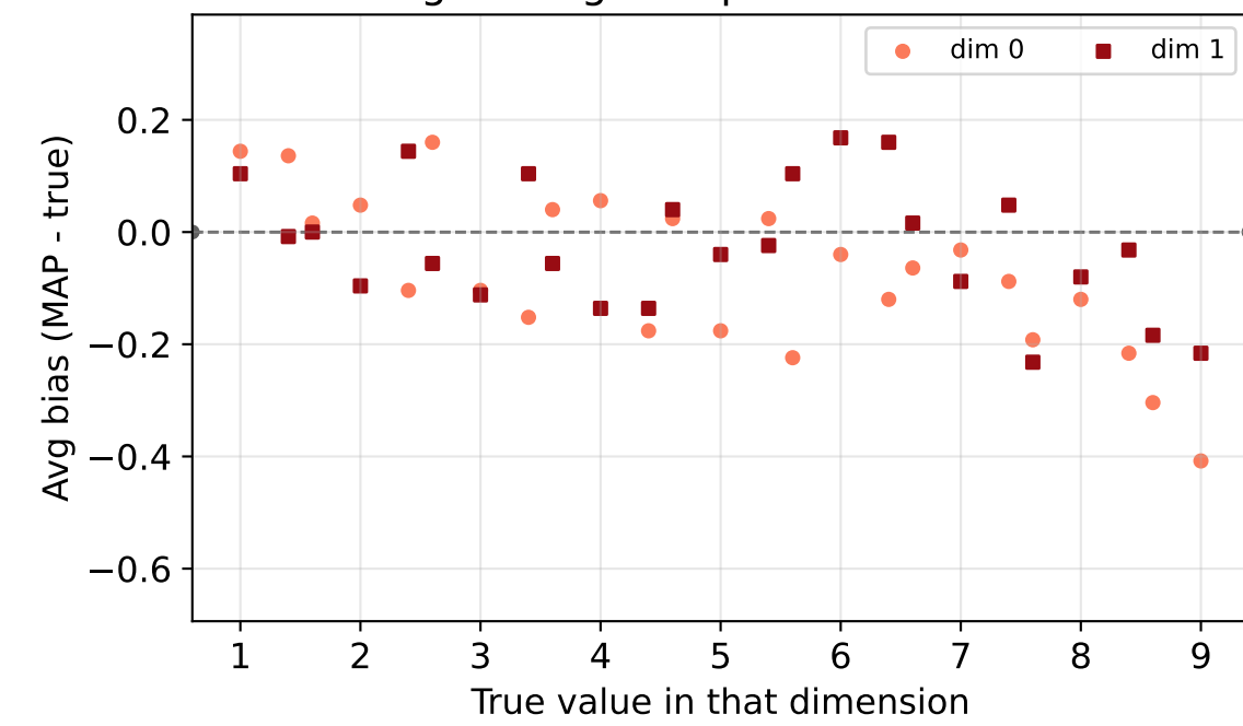
exponential: avg bias per dimension
