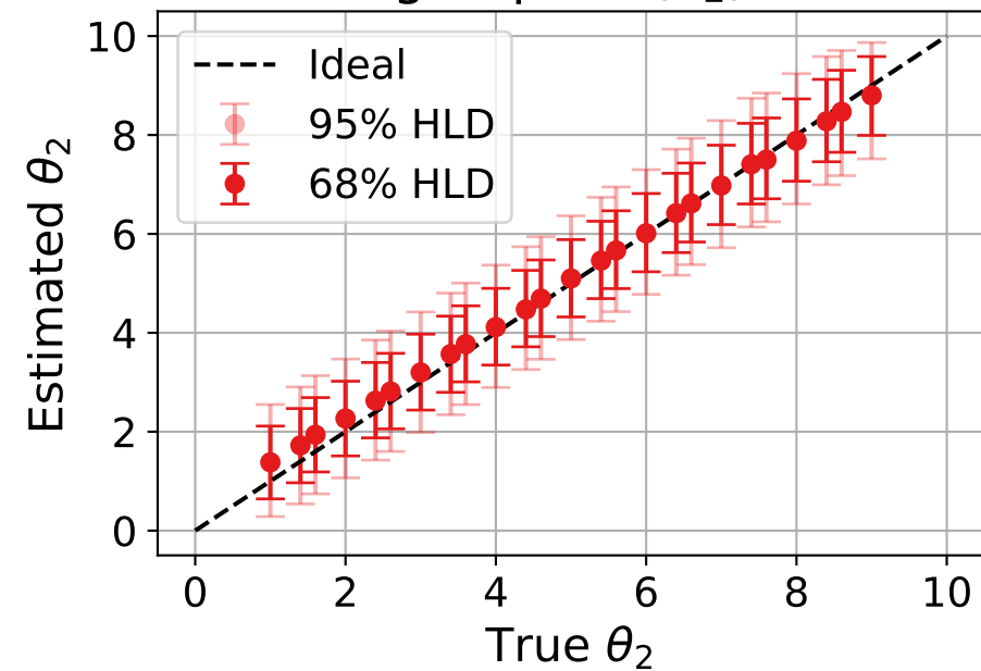
grid prior ( \theta_2 )
