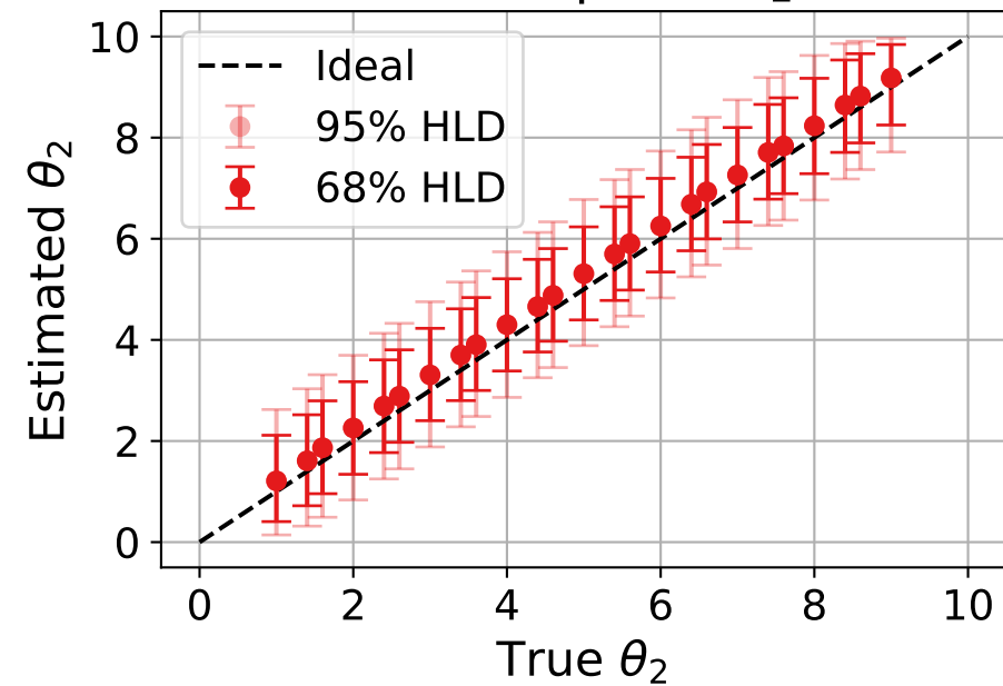
uniform prior ( \theta_2 )
