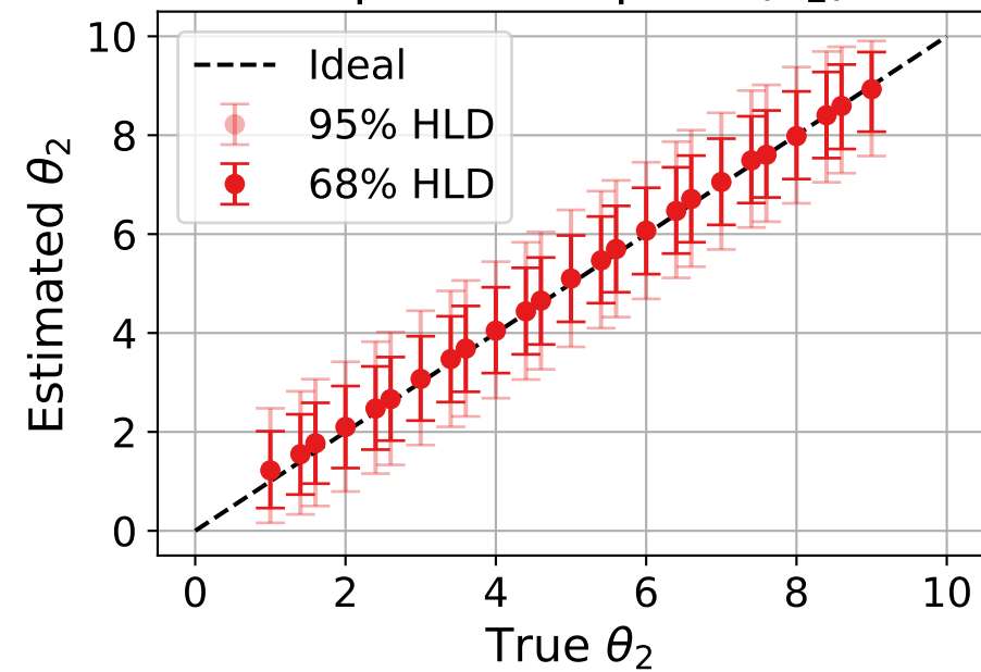
exponential prior ( \theta_2 )
