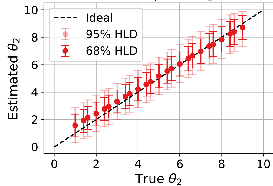
normal prior ( \theta_2 )
