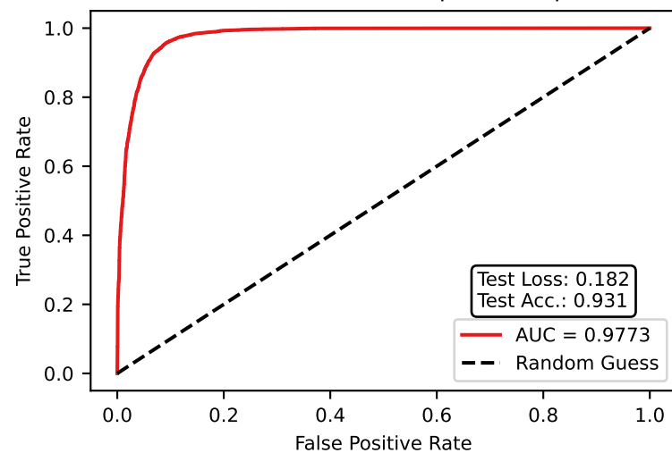
Test ROC Curve for 0. exponential prior
