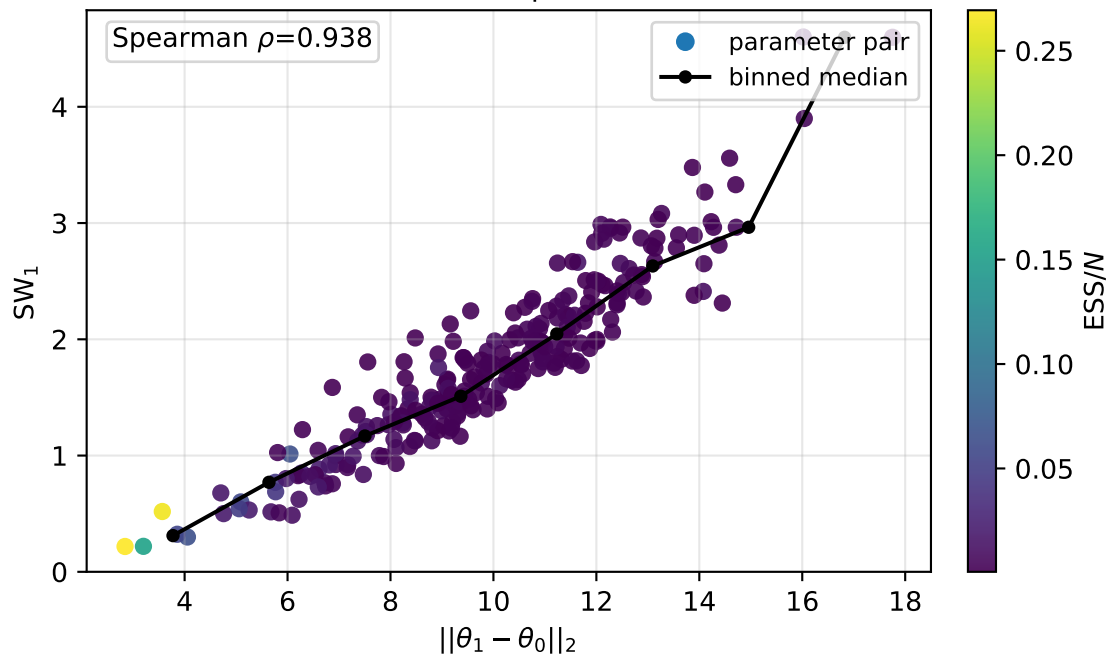
normal prior median=1.67 | worst=4.53
