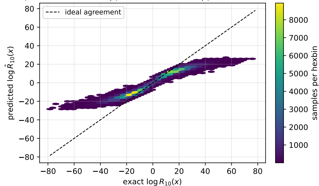
grid prior
