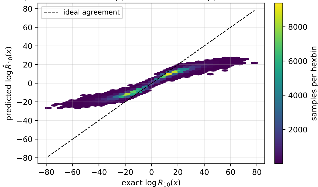
exponential prior
