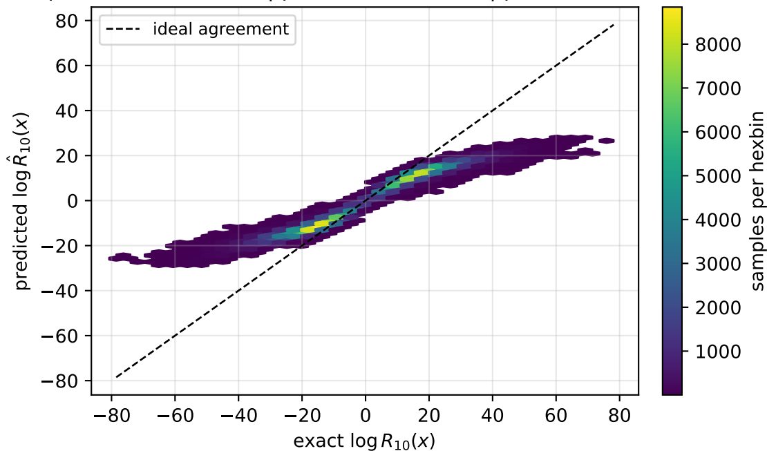
exponential prior
