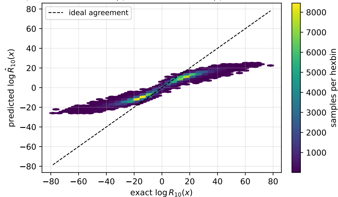
grid prior
