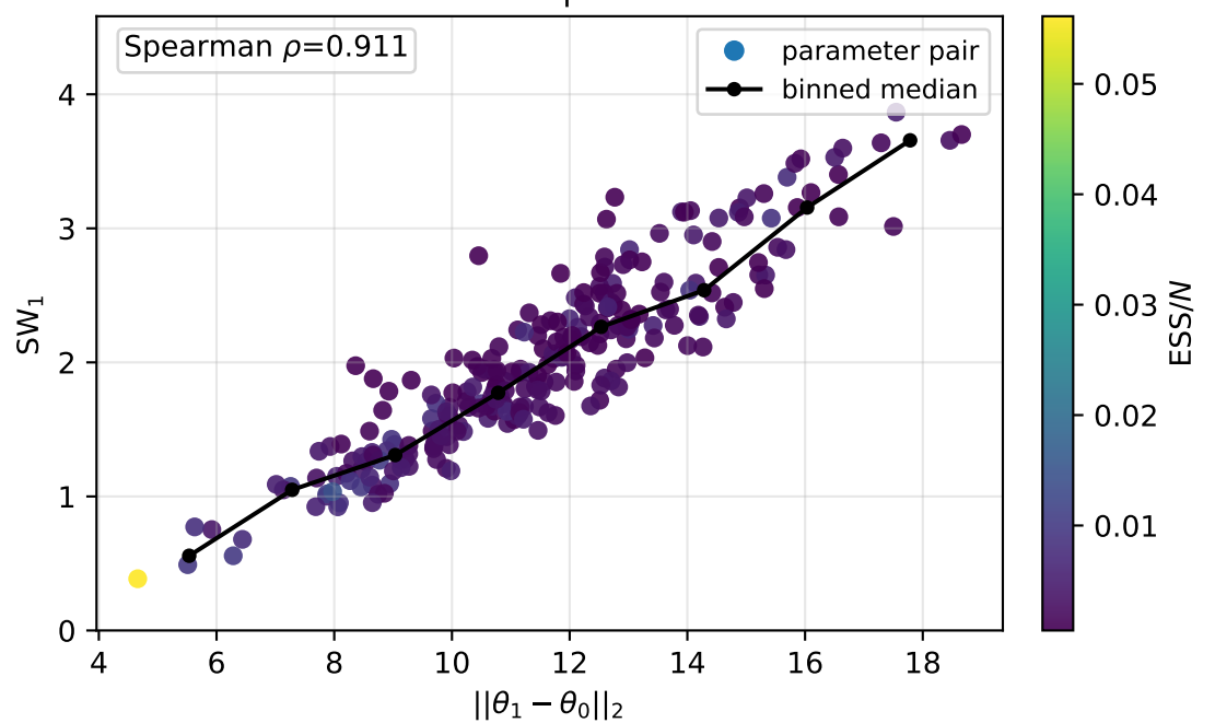
exponential prior median=1.94 | worst=3.87
