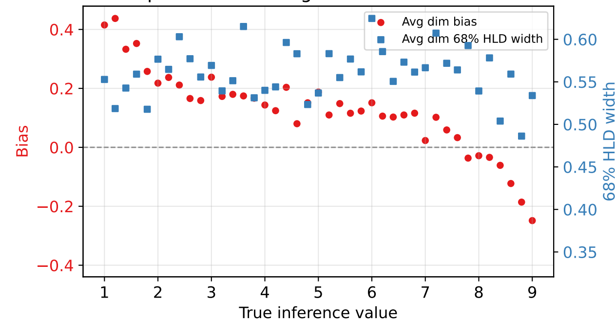
grid: averages across dimensions
