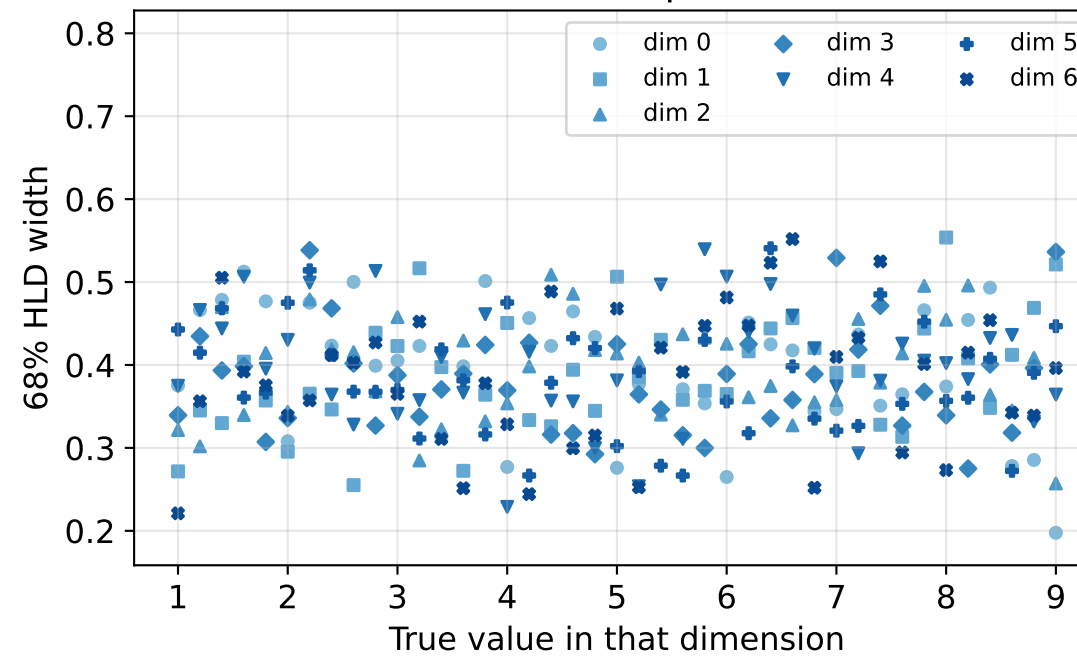
exponential: HLD width per dimension
