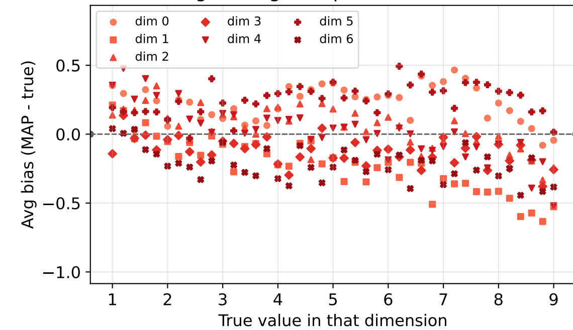
grid: avg bias per dimension
