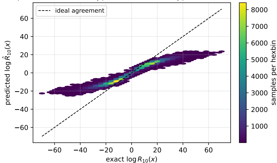
exponential prior pooled RMSE=7.57 | pair median=5.67 | pair worst=24.2
