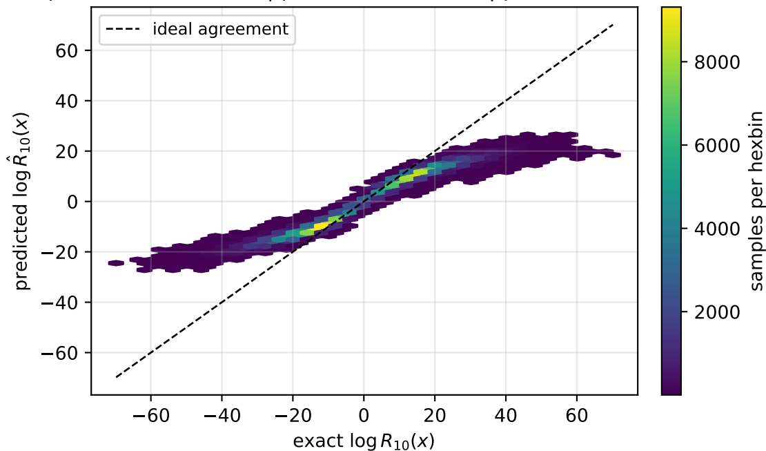
uniform prior pooled RMSE=6.89 | pair median=4.89 | pair worst=23.7
