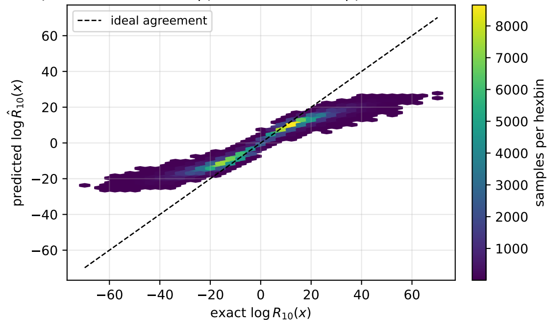
normal prior pooled RMSE=6.73 | pair median=4.8 | pair worst=22.5
