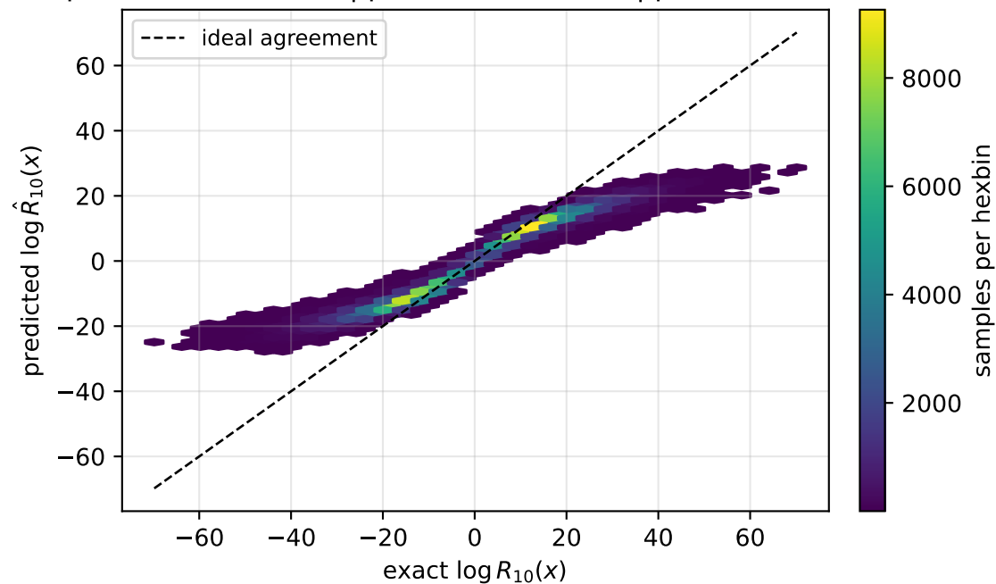
grid prior pooled RMSE=6.22 | pair median=4.22 | pair worst=20.6
