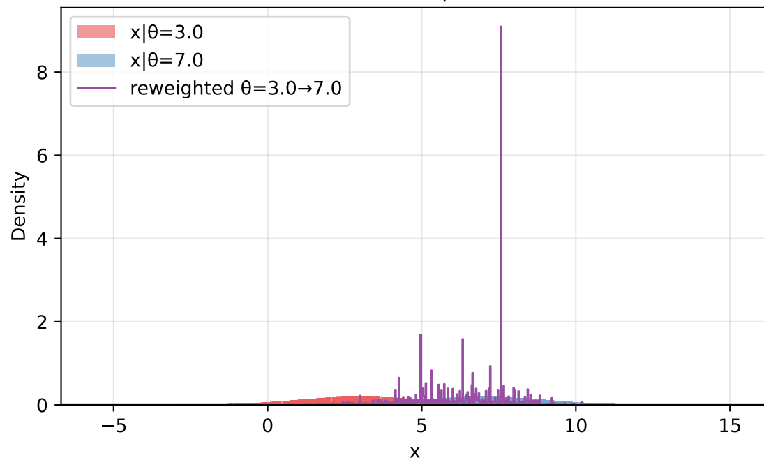
exponential prior N=1,000,000 | ESS=21
