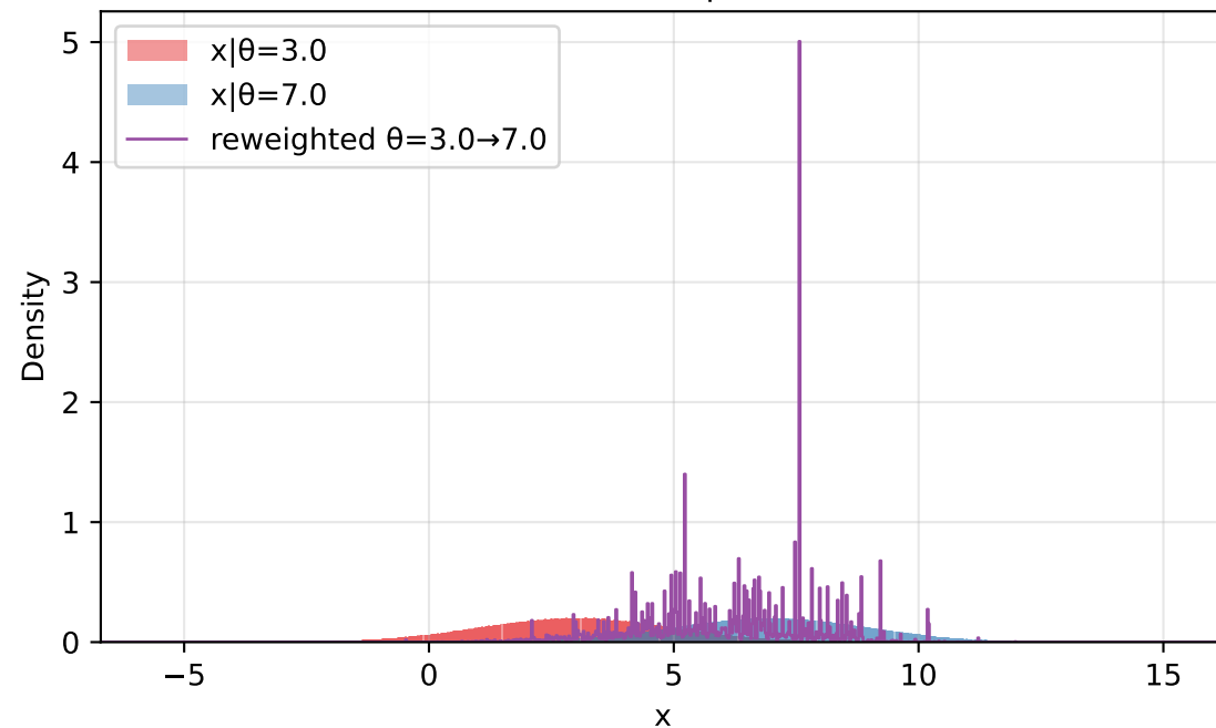
grid prior N=1,000,000 | ESS=23
