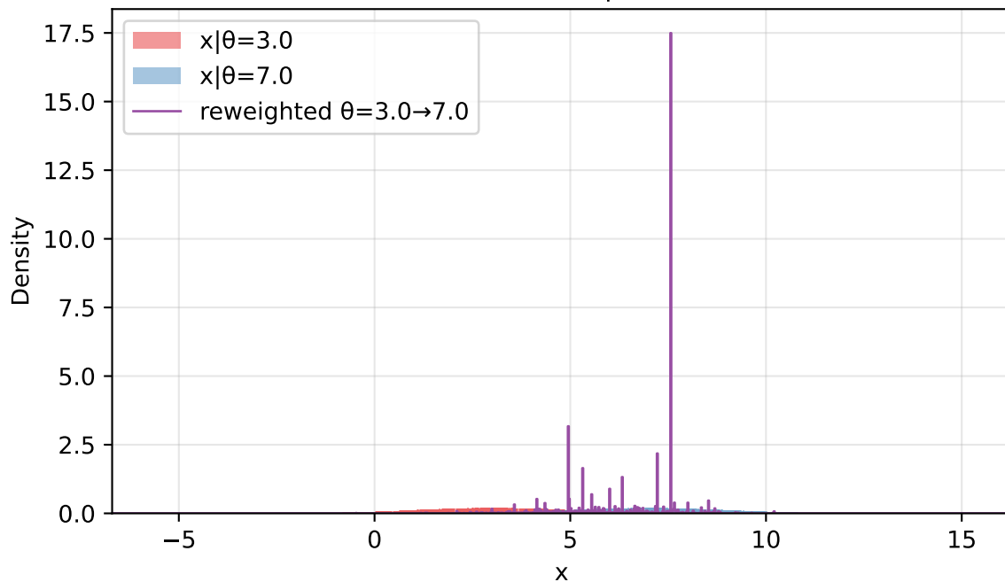
exponential prior N=1,000,000 | ESS=21
