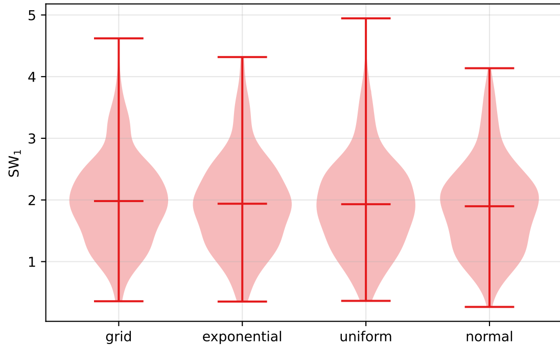
SW 1 by prior
