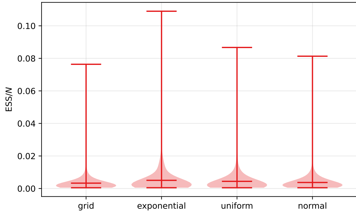
ESS/N by prior
