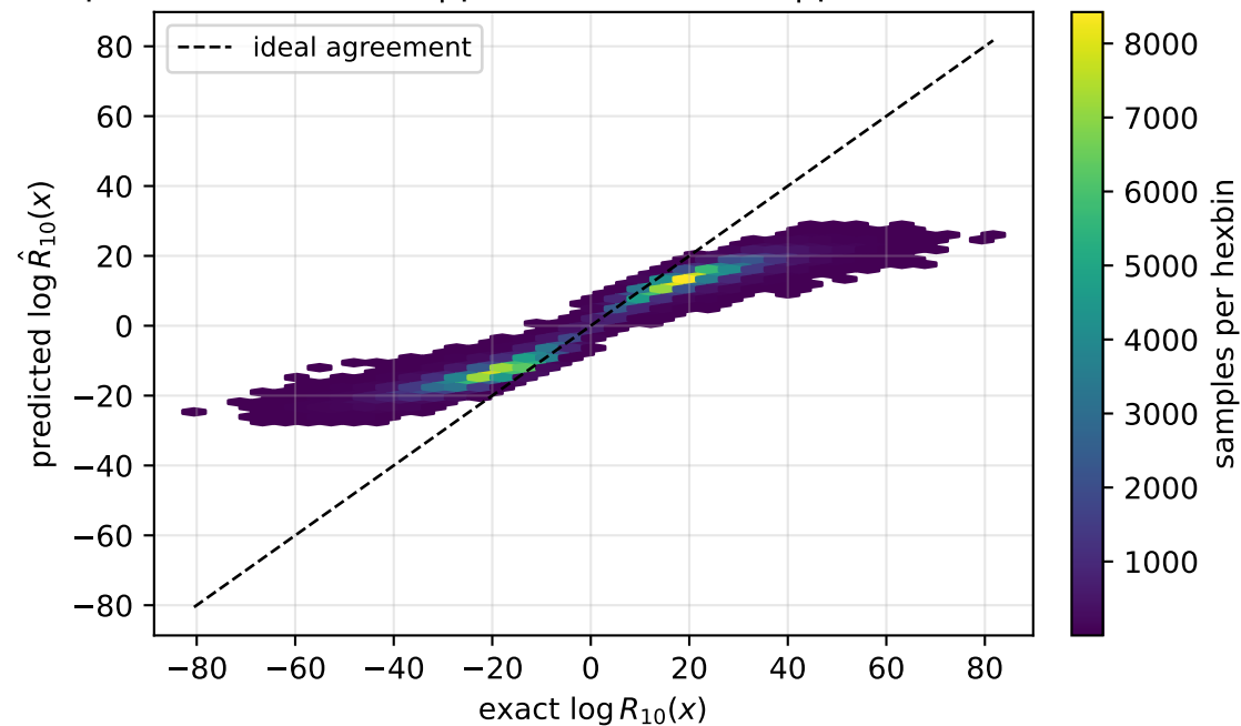
grid prior pooled RMSE=9.48 | pair median=7.59 | pair worst=26.7
