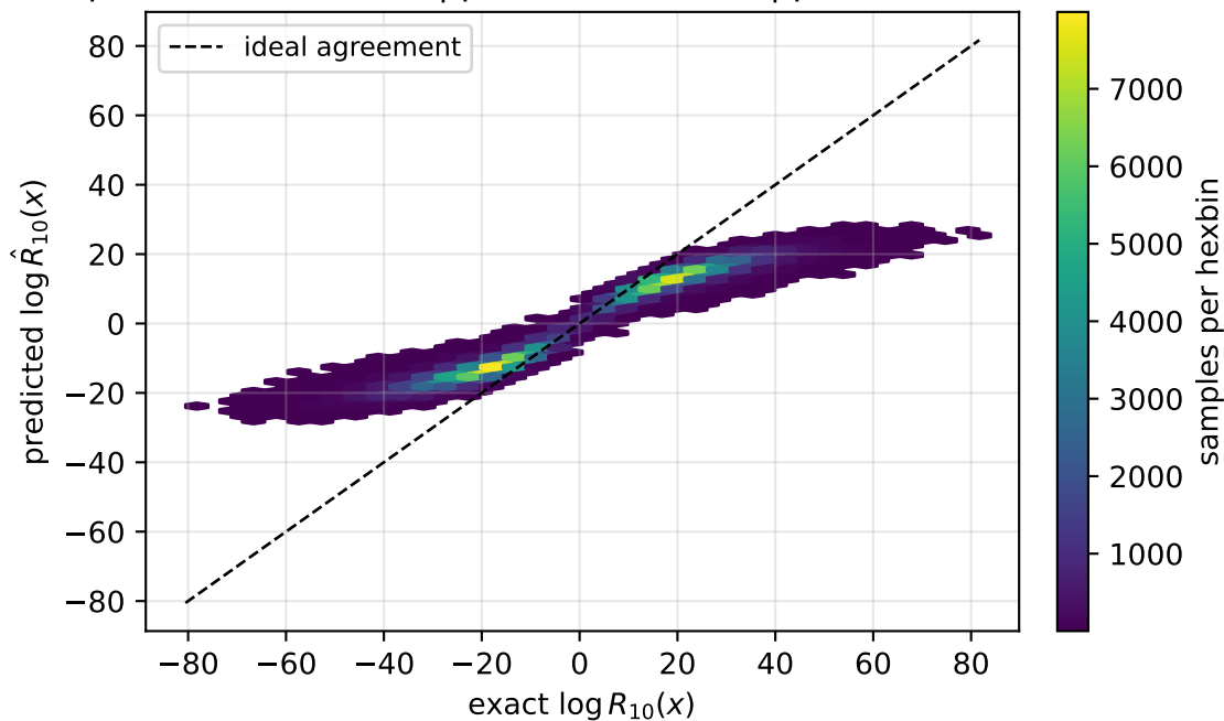
exponential prior pooled RMSE=9.59 | pair median=7.6 | pair worst=27.4
