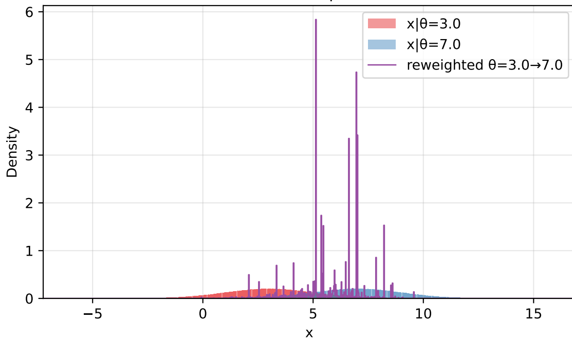
exponential prior N=1,000,000 | ESS=23
