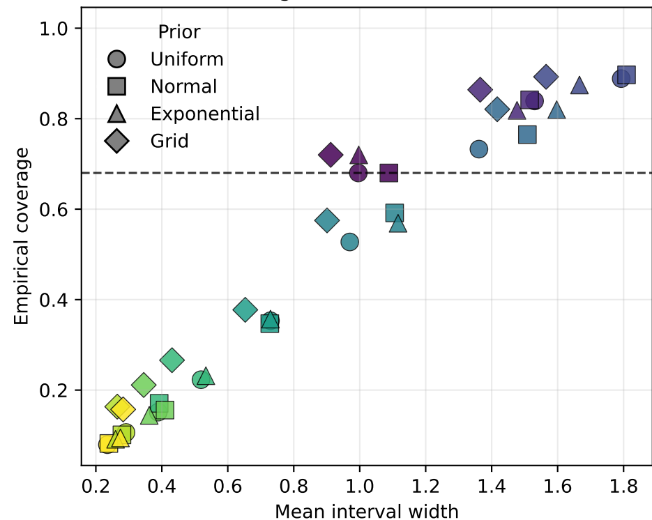
Coverage vs width (68% HLD)
