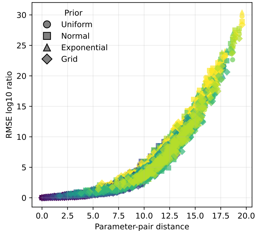
Distance vs RMSE log10 ratio
