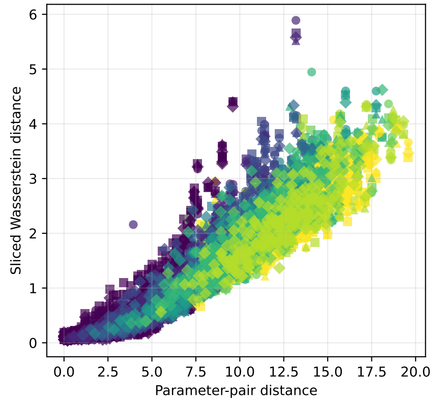
Distance vs Sliced Wasserstein distance
