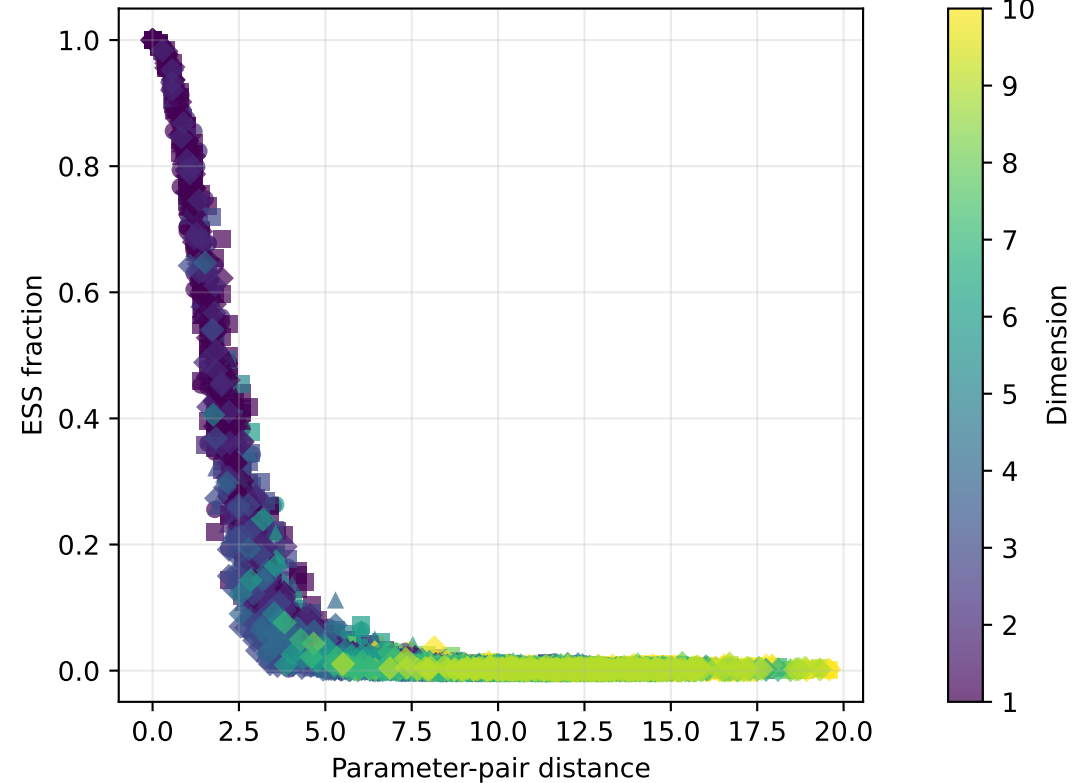
Distance vs ESS fraction
