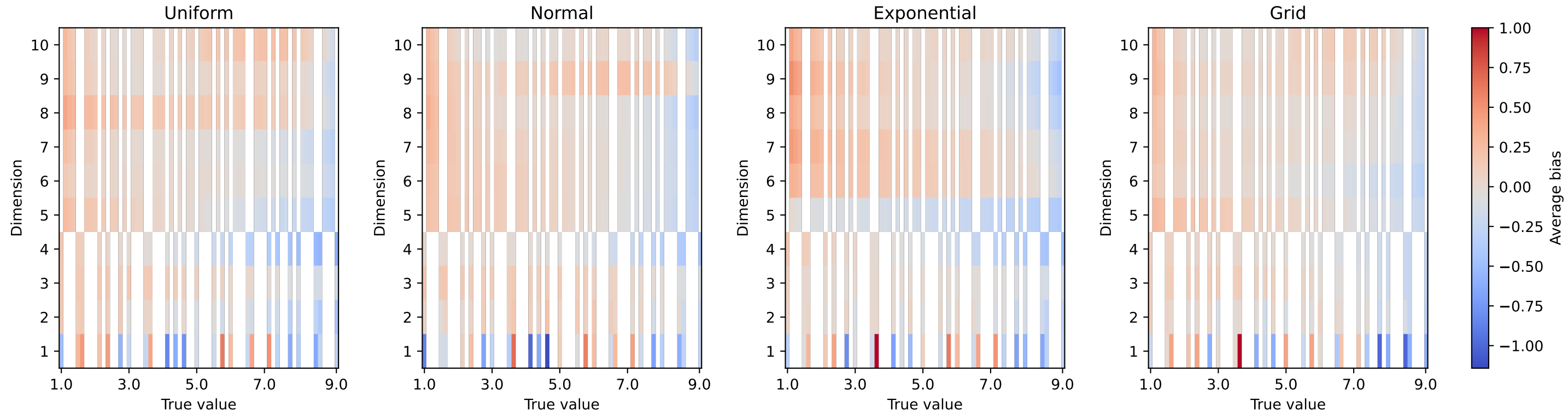
Bias heatmaps by prior
