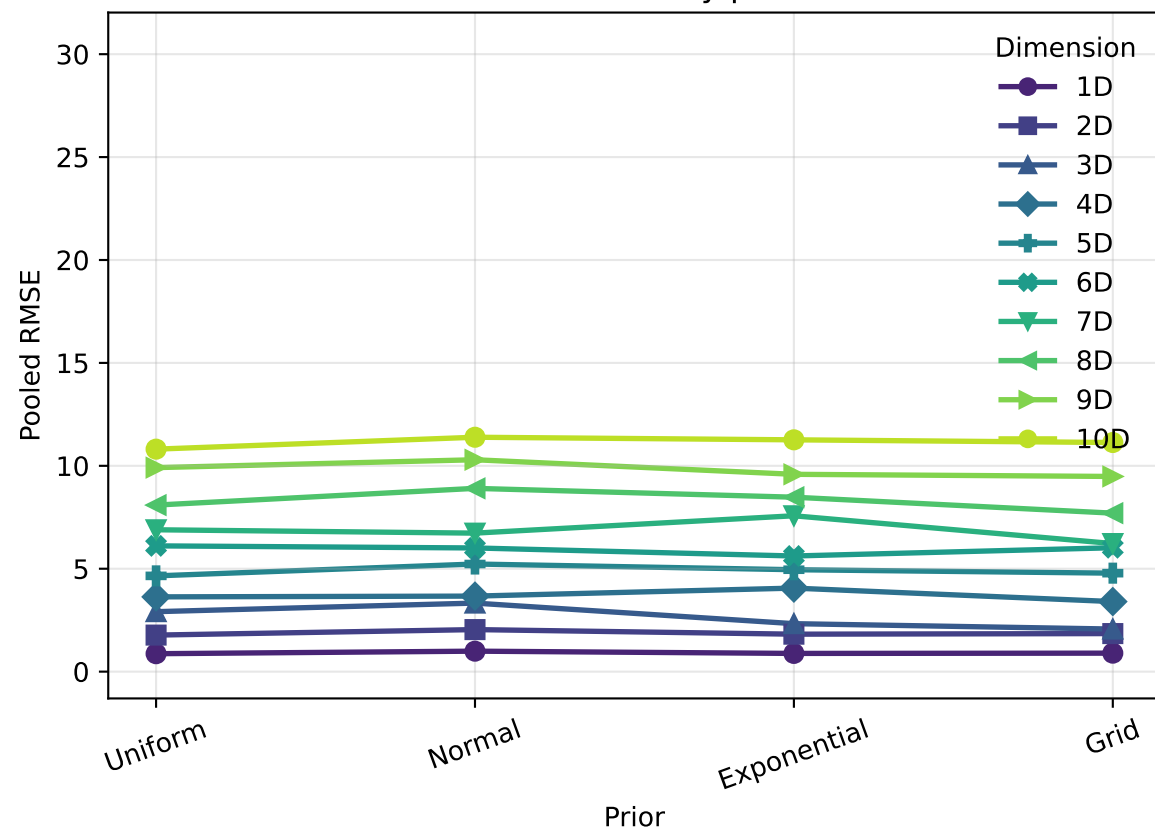
Pooled RMSE by prior
