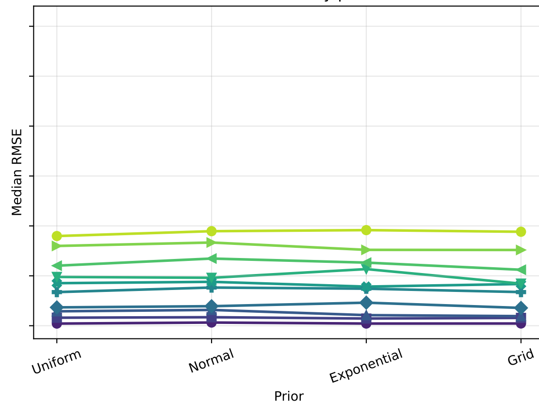
Median RMSE by prior
