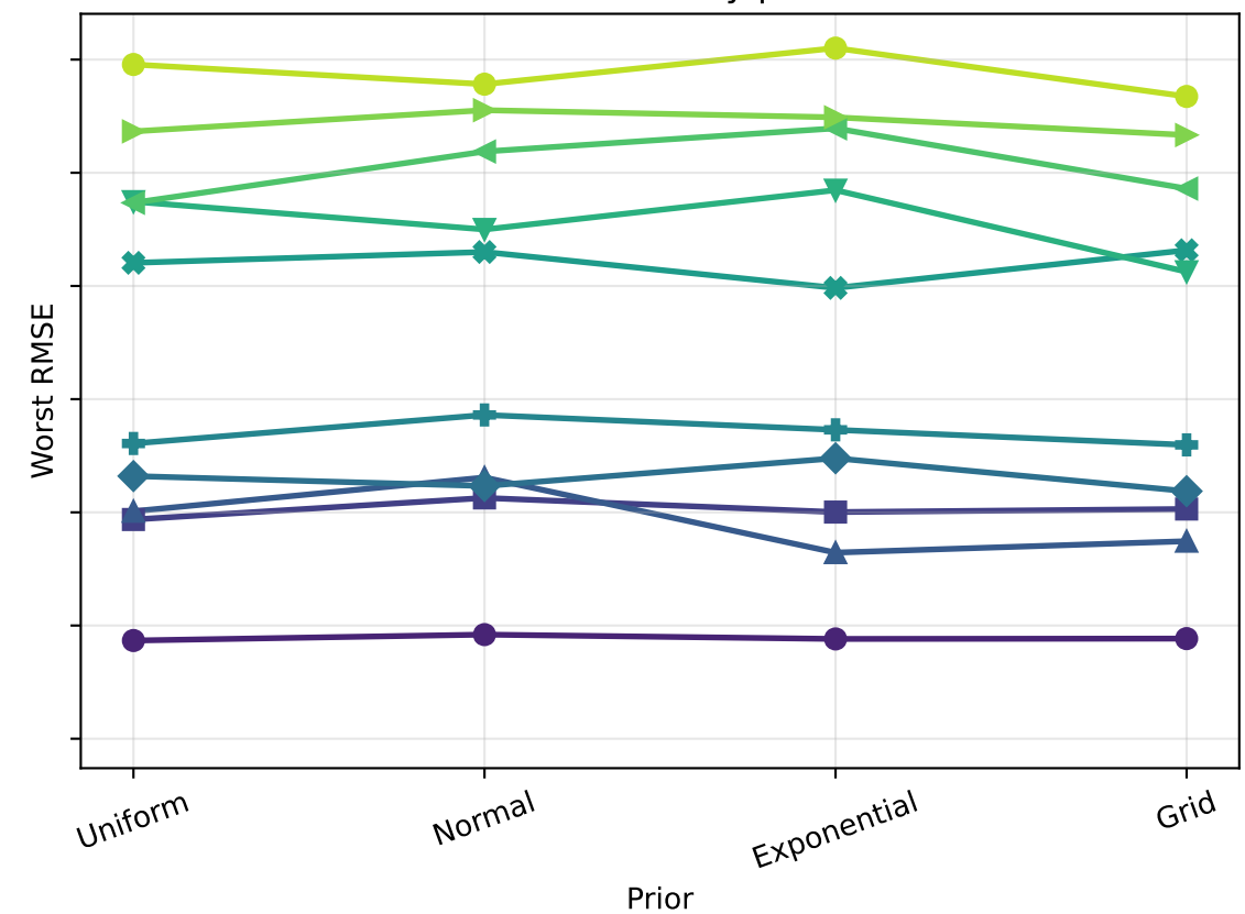
Worst RMSE by prior
