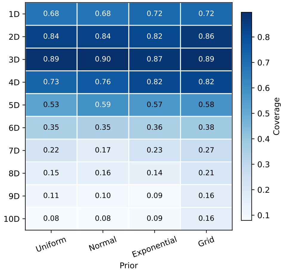
68% HLD coverage
