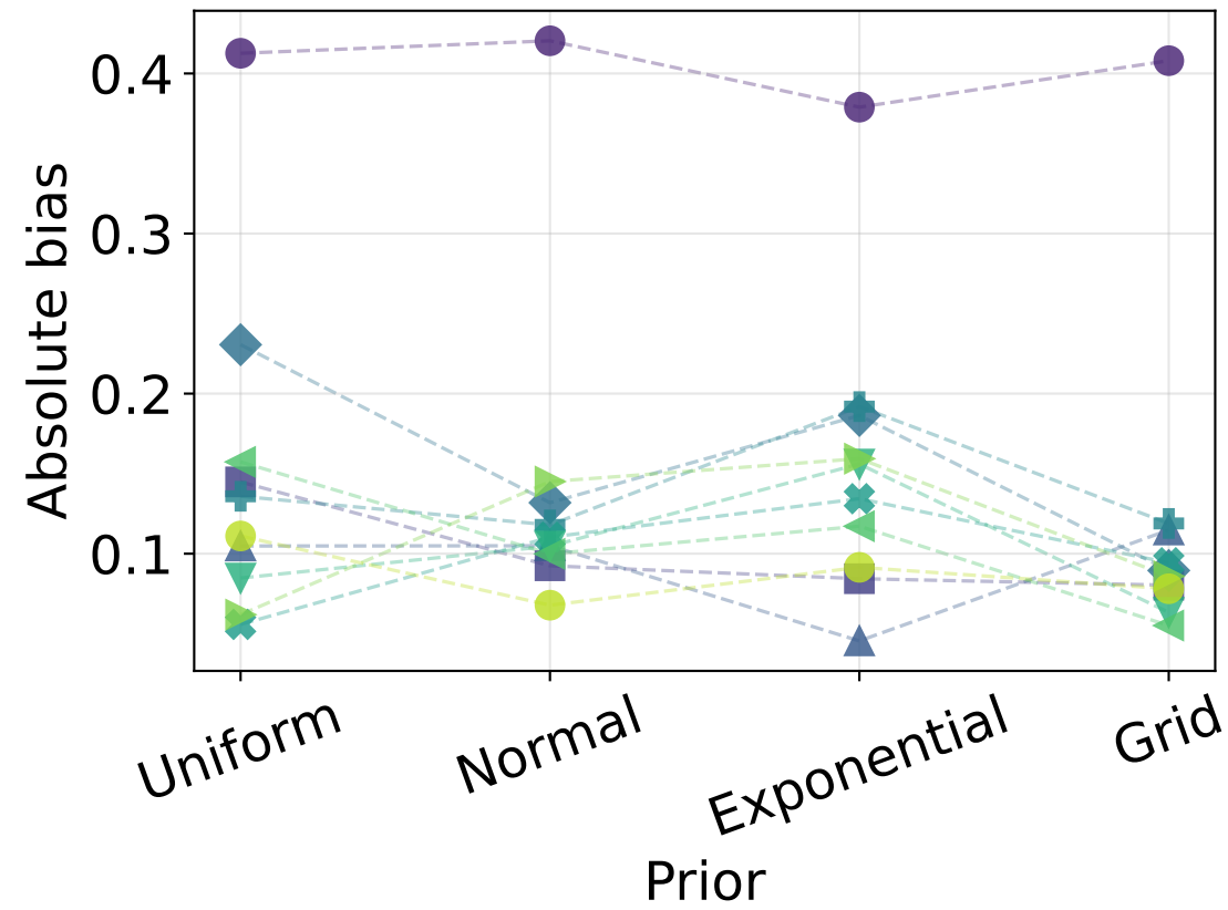
Mean absolute bias
