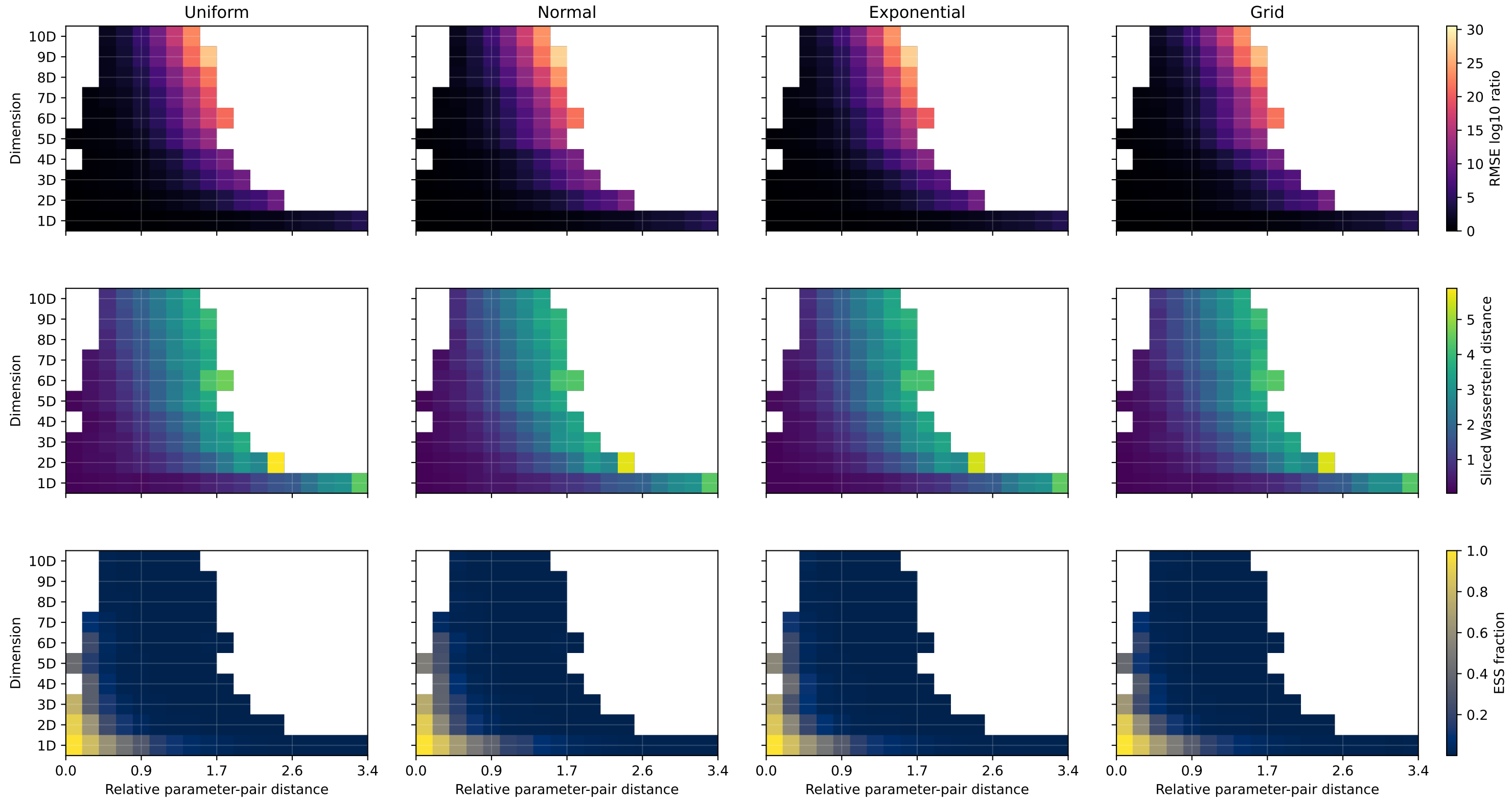
Distance-driven difficulty heatmaps by prior Distance normalized by the median within each dimension-prior slice
