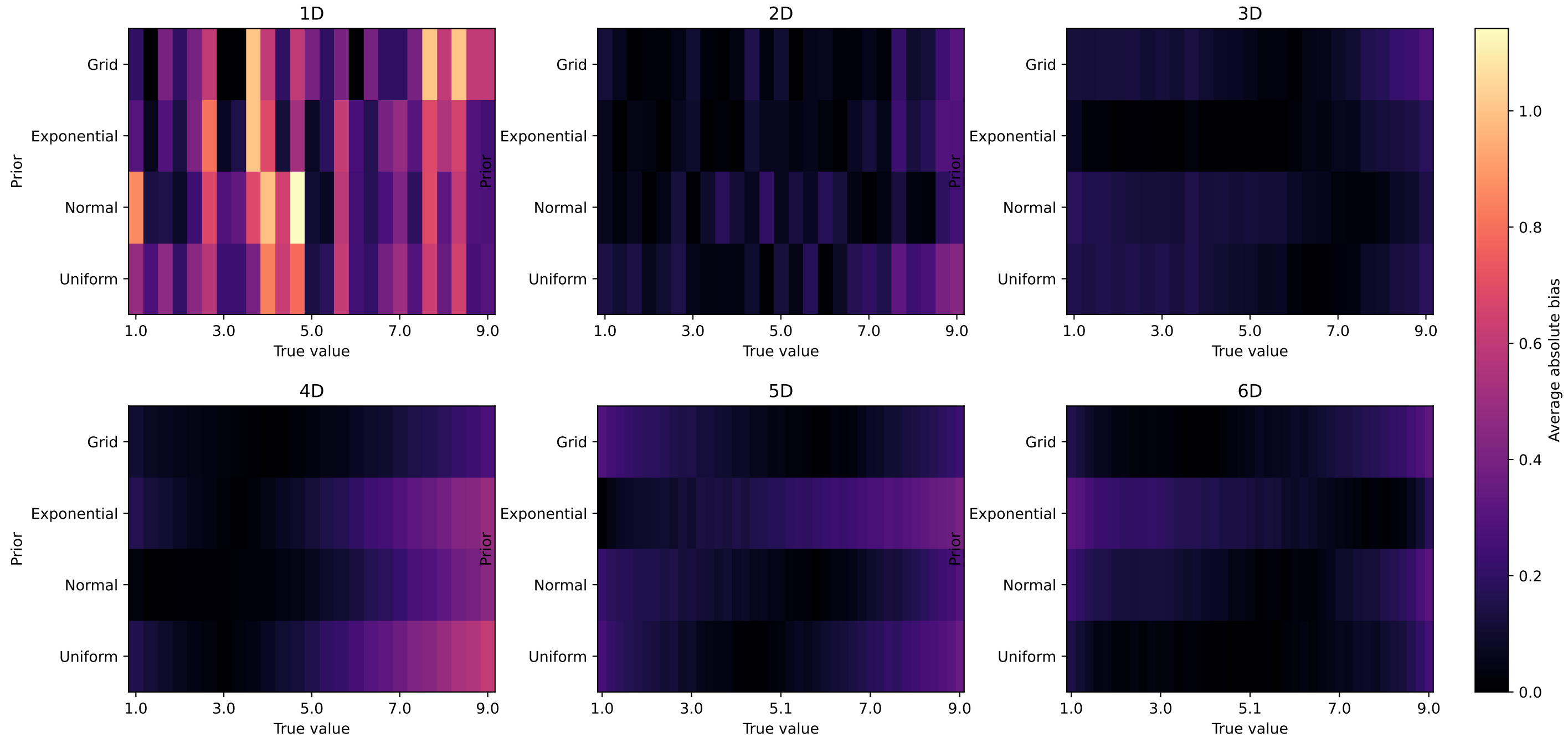
Absolute bias heatmaps with prior rows
