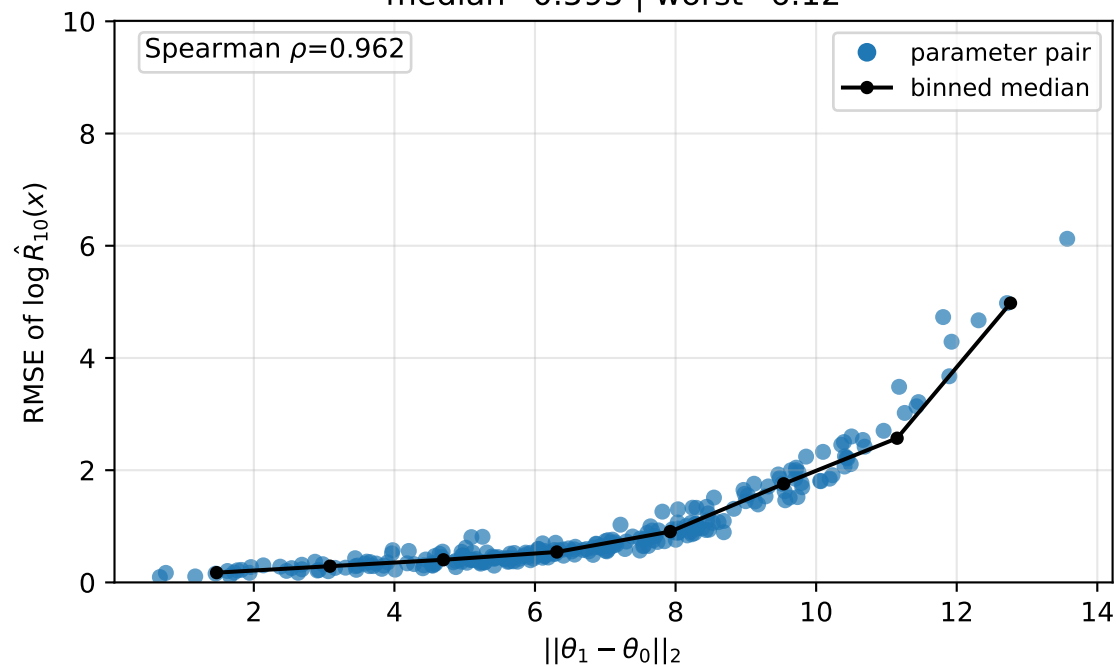
exponential prior median=0.595 | worst=6.12
