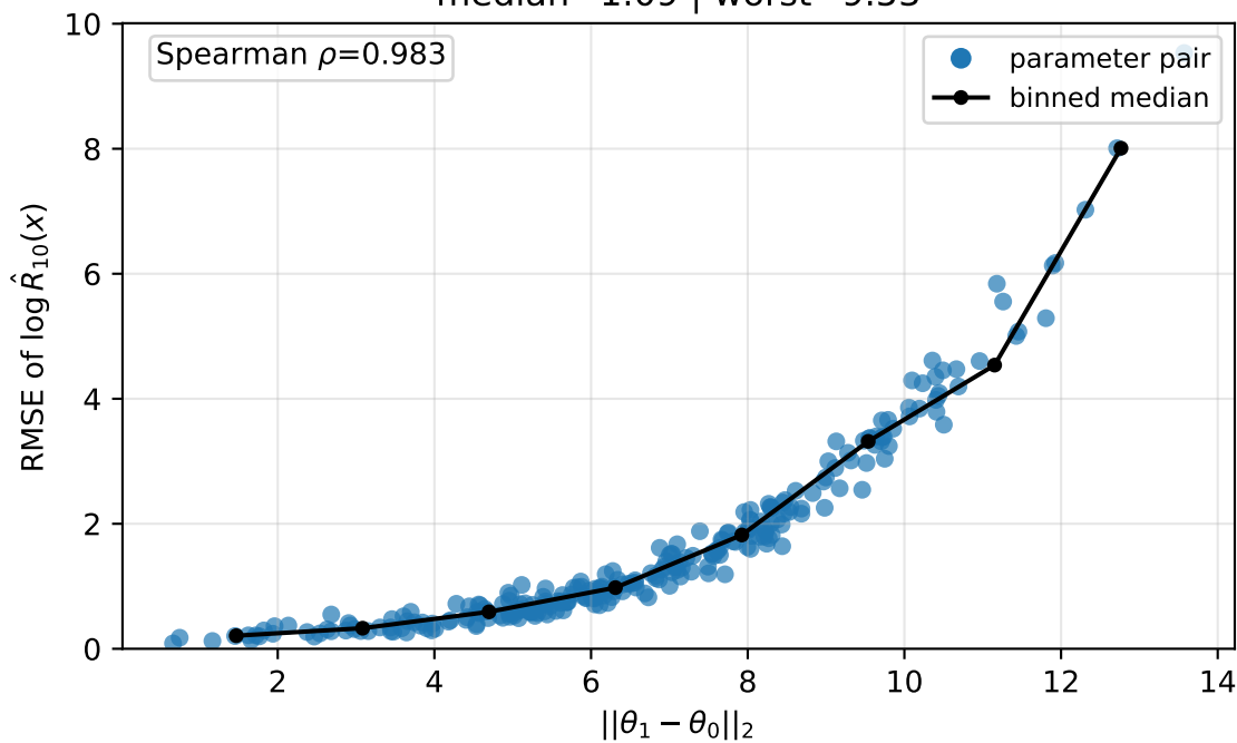
normal prior median=1.09 | worst=9.53
