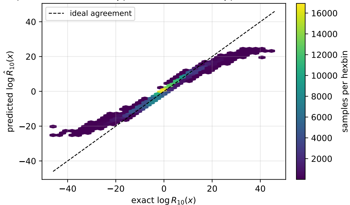
exponential prior pooled RMSE=1.28 | pair median=0.595 | pair worst=6.12
