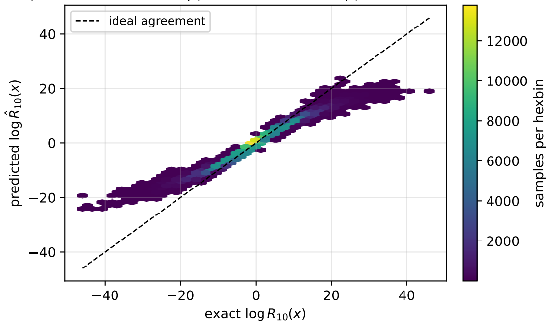
normal prior pooled RMSE=2.19 | pair median=1.09 | pair worst=9.53
